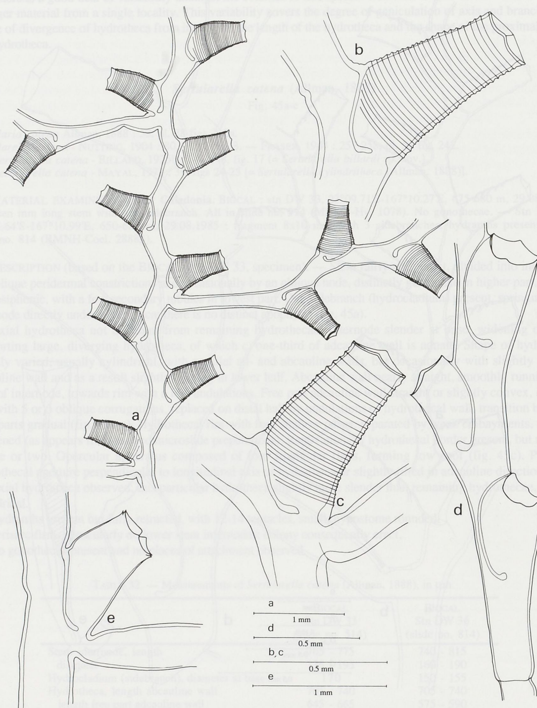
FIG. 46 a-c. — Sertularella crenulata Nutting, 1905, MUSORSTOM 4, Stn CP 193 : a, monosiphonic distal part of colony; b, hydrocladial hydrotheca; c, axillary hydrotheca. FIG. 46 d. — Sertularella diaphana (Allman, 1885), BIOCAL, Stn DW 36, part of hydrocladium. FIG. 46 e. — Sertularella geodiae Totton, 1930, BIOGEOCAL, Stn CP 214, axillary hydrotheca. a-c, slide no. 345; d, slide no. 488; e, slide no. 581.
