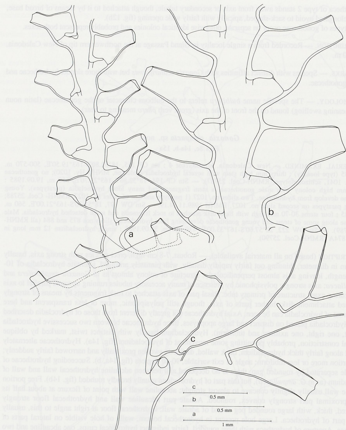
FIG. 14 a-b. — Gonaxia compacta sp. nov.: a, schizoholotype, MUSORSTOM 4, Stn CP 155, insertion of hydrocladium on axis; b, paratype, part of hydrocladium.
