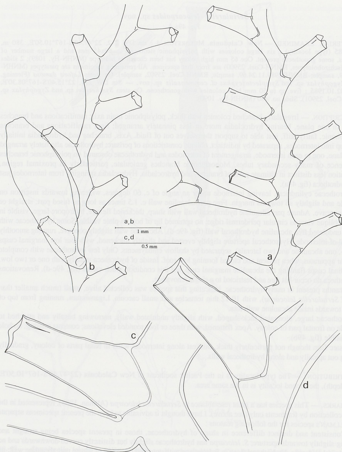
FIG. 49. — Sertularella leiocarpoides sp. nov., schizoholotype, MUSORSTOM 4, Stn DW 212 : a, monosiphonic distal part of axis; b, monosiphonic part of axis with gonotheca; c, axillary hydrotheca; d, hydrocladial hydrotheca. a-d, slide no. 347.
