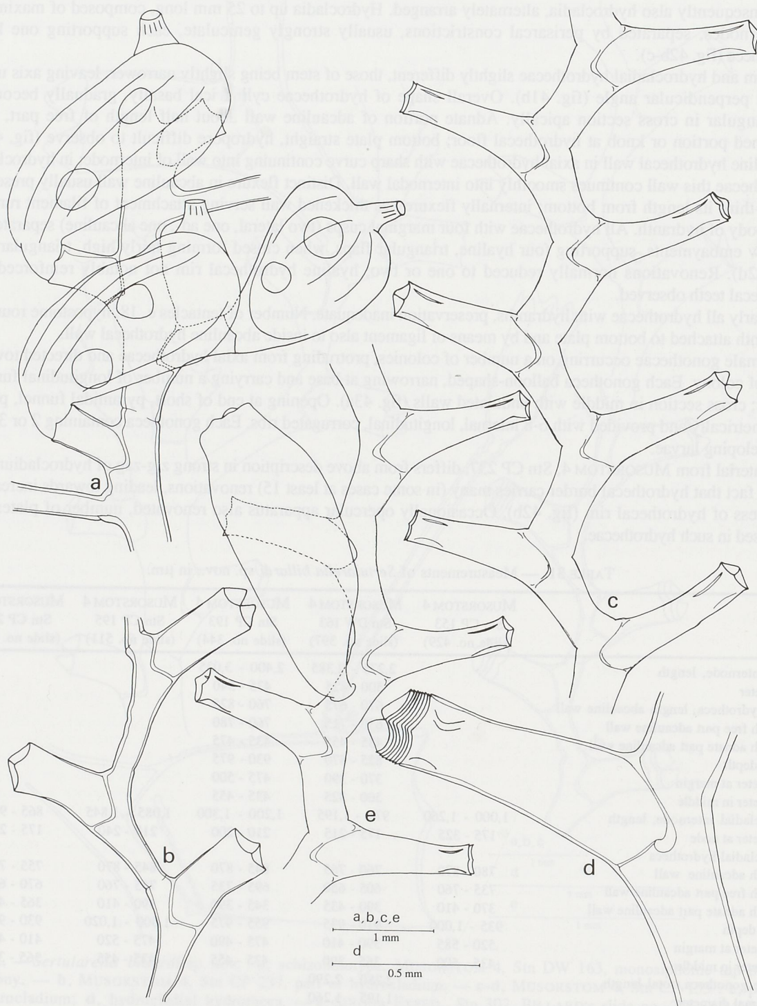
FIG. 43 a-b. — Sertularella billardi sp. nov. : a, schizoholotype, MUSORSTOM 4, Stn DW 163, part of axis with gonothecae (pressed aside by cover glass). — b, MUSORSTOM 4, Stn CP 193, part of hydrocladium. FIG. 43 c-e. — Sertularella bipectinata sp. nov. : c-d, BIOCAL, Stn DW 36 : c, schizoholotype, part of axis; d, axial hydrotheca. — e, MUSORSTOM 4, Stn DW 220, part of axis with gonotheca. a, slide no. 397; b, slide no. 492; c, slide no. 485; d, slide no. 497; e, slide no. 515.
