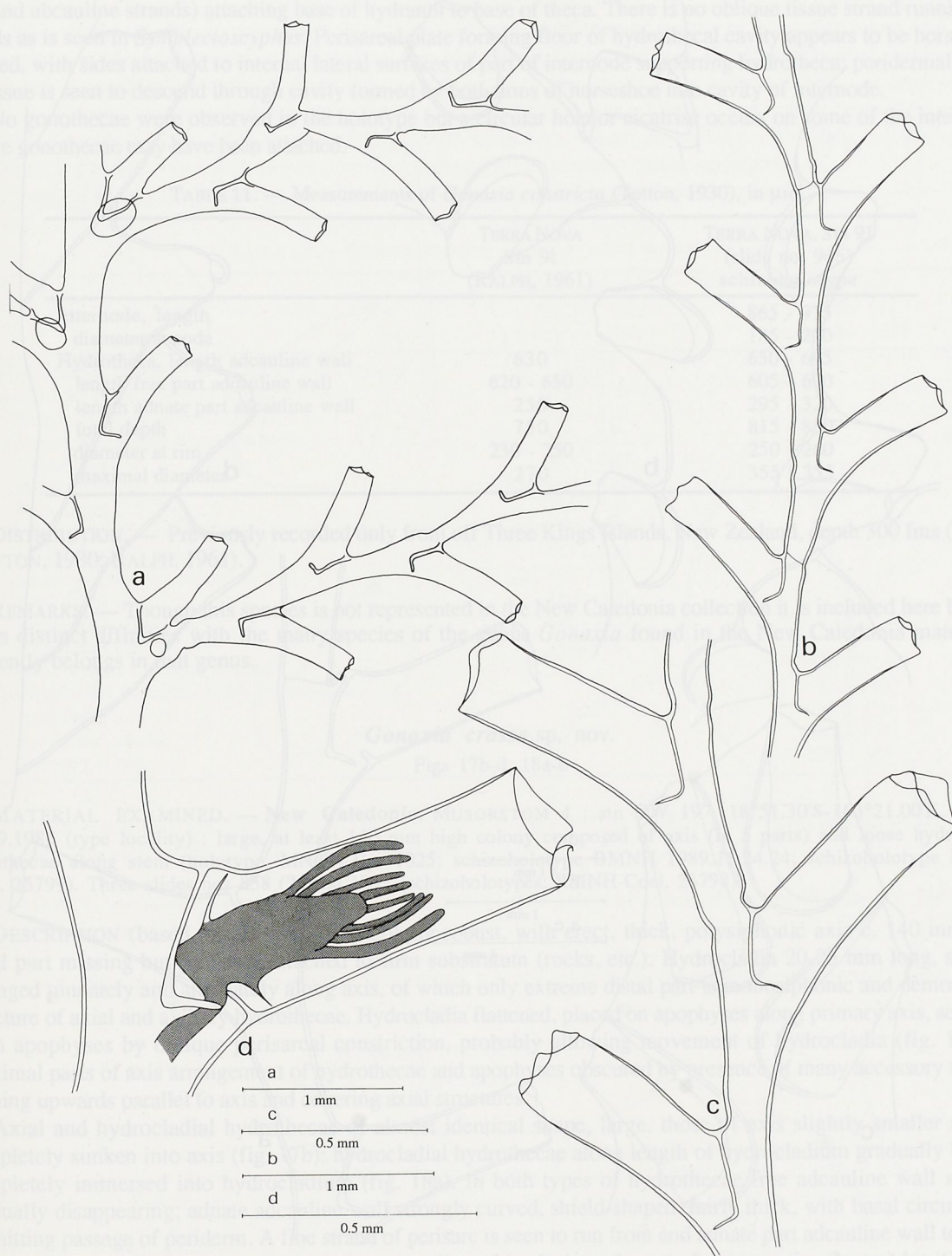
FIG. 16 a-c. — Gonaxia complexa sp. nov., BIOCAL, Stn DW 08 : a, top part of colony; b, part of hydrocladium; c, three hydrothecae from hydrocladium.
