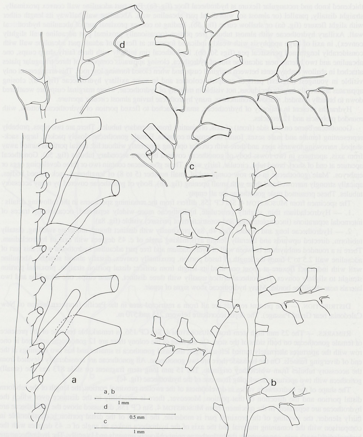
FIG. 5. — Gonaxia amphorifera sp. nov., paratypes, MUSORSTOM 4, Stn CP 153 : a, female gonothecae, lateral view, semi-diagrammatic; b, male gonothecae, frontal view; c, origin of hydrocladium on axis; d, axillary hydrotheca. a, slide no. 1016; b, slide no. 856; c, d, slide no. 1017.
