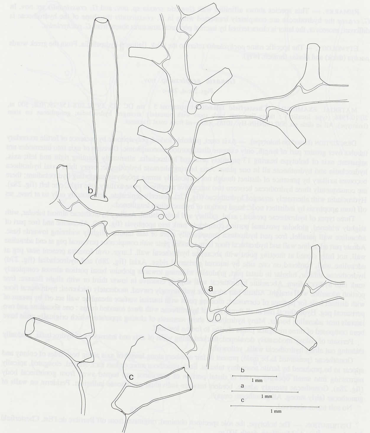
FIG. 29 a-b. — Gonaxia persimilis sp. nov., BIOGEOCAL, Stn DW 291 : a, monosiphonic distal part of colony; b, female gonotheca.
