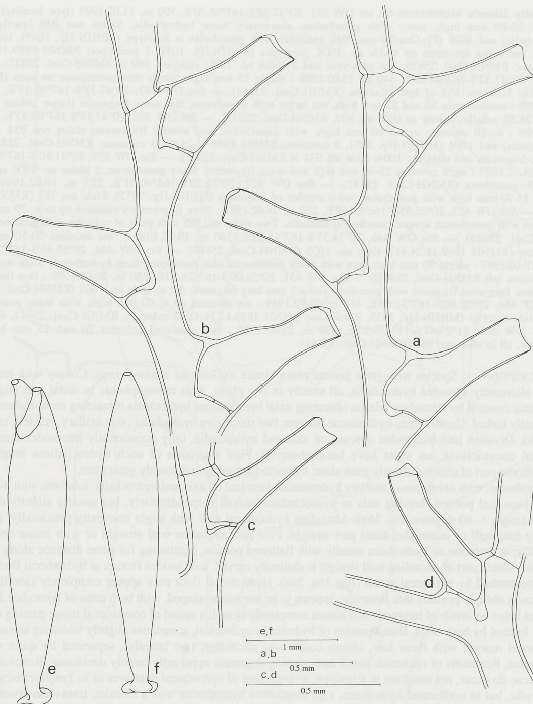
FIG. 33 a-b. — Gonaxia persimilis sp. nov.: a, BIOGEOCAL, Stn DW 291, part of hydrocladium. — b, MUSORSTOM 6, Stn DW 461, part of hydrocladium.
