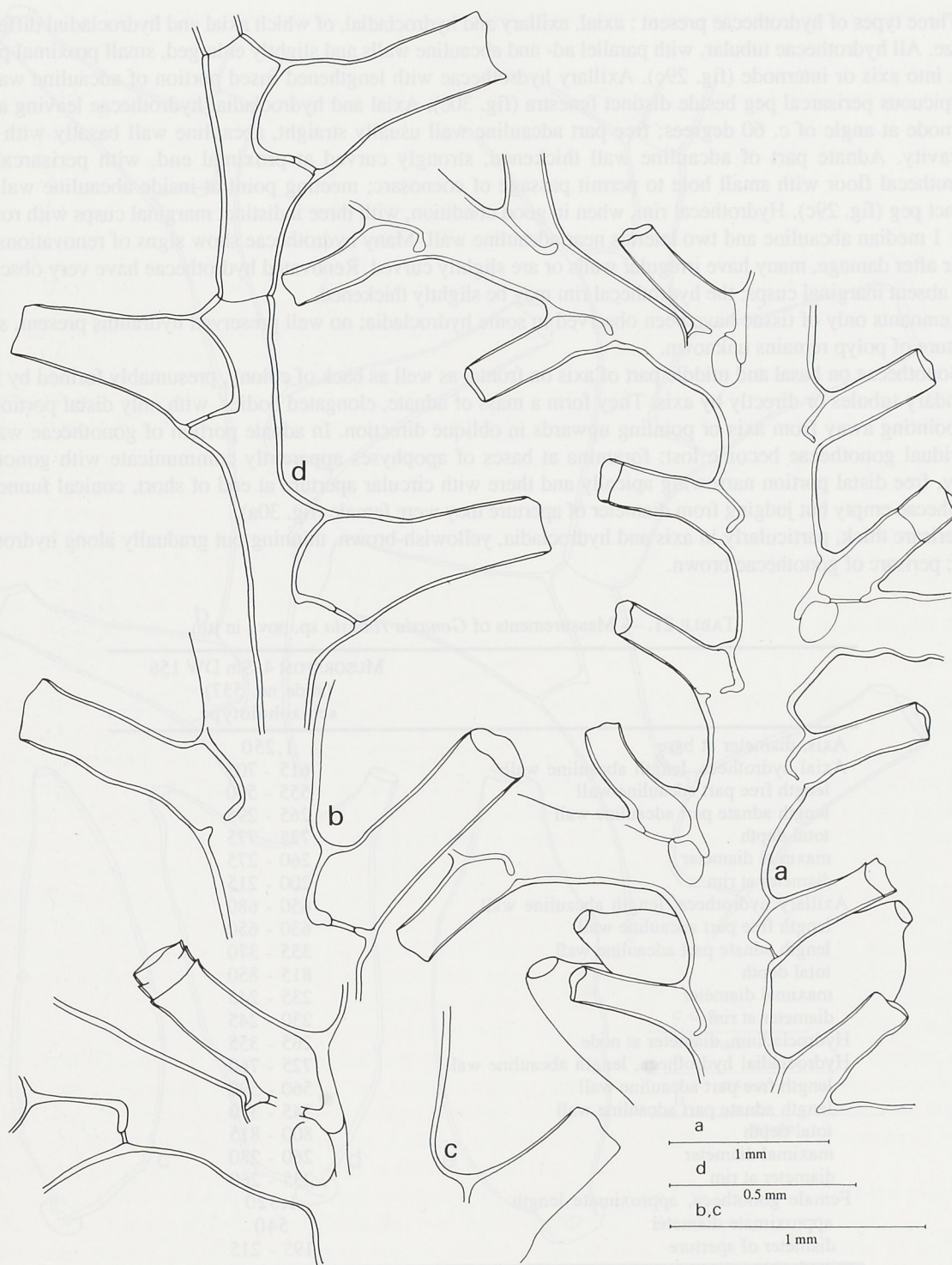
FIG. 30 a-c. — Gonaxia robusta sp. nov., schizoholotype, MUSORSTOM 4, Stn DW 156 : a , monosiphonic distal part of colony, frontal view; gonothecae on backside; b , hydrocladial hydrothecae; c , axillary hydrotheca. FIG. 30 d. — Gonaxia persimilis sp. nov., CHALCAL 2, Stn DW 76, part of hydrocladium. a-c, slide no. 537; d, slide no. 532.
