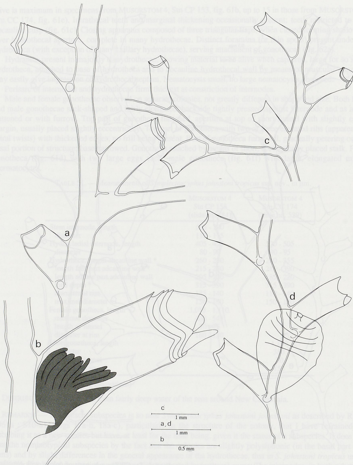
FIG. 63. — Symplectoscyphus paulensis Stechow, 1923 : a-b, lectotype, VALDIVIA, Stn 165, 38°40'S-77°39'E : a, monosiphonic upper part of axis; b, hydrocladial hydrotheca with its hydranth. — c-d, SAM, ABD 8C, 24°40'S-35°28'E : c, top part of colony; d, part of axis with (flattened) gonotheca.
