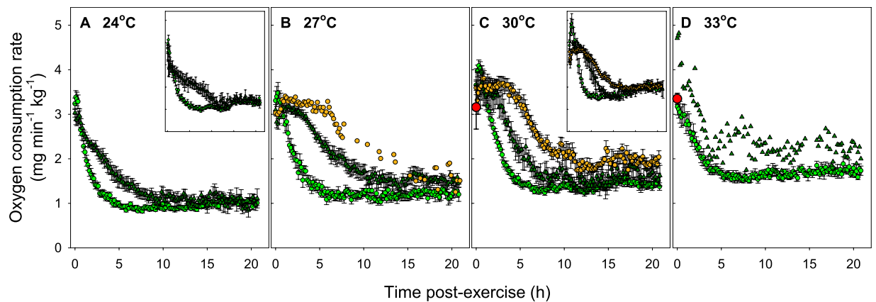
Figure 1. Recovery in the oxygen consumption rate (means \pm SE) of coral grouper following the burst-exercise fishing simulation in fully-acclimated fish (i.e., ~6 weeks) at (A) 24°C, (B) 27°C, (C) 30°C, and (D) 33°C. Insets in (A) and (C) show data for early-acclimated fish (i.e., 2–3 weeks). Survivors are separated into fish that achieved exercise performance scores of \leq 3 (light green circles) and those with scores > 3 (dark green triangles). Delayed mortalities are presented as orange circles. Short-term mortalities died within respirometers and thus only the first post-exercise measurement was taken for each fish (large red circles). Sample sizes given in Fig. 3.
