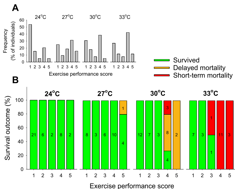
Figure 3. Frequency distributions of exercise performance scores (A) and survival outcomes as a function of exercise performance scores (B) of coral grouper in the four temperature treatment groups. Green, orange and red colouration represents survivors, delayed mortalities and short-term mortalities, respectively. Sample sizes are given in the bars of (B). For visual clarity, exercise performance scores were rounded down such that a score of 3.5 became 3.0, etc. For individuals that were tested in the early-acclimation group as well as following full acclimation (subsets in the 24 and 30 °C groups; Table 1), the trial after full thermal acclimation is the one included here. However, four fish from the early-acclimation group at 30 °C had exercise performance scores \geq 4 and suffered delayed mortality (Table 1), and thus are included here.
