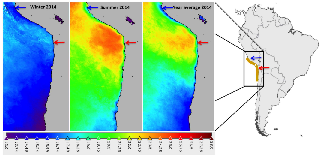
Figure 3. Sea surface temperature (sst) in the distribution range of Ectocarpus sp. for year 2014. The blue arrow represents the original location of the male parent (San Juan de Marcona, Peru) and the red arrow represents the original location of the female parent (Arica, Chile). Created with the SeaWiFS Data Analysis System (SeaDAS) visualization and data processing software version 7.2, using seasonal (winter and summer) and annual MODIS sst data from 2014: http://seadas.gsfc.nasa.gov/installers/ ; http://oceandata.sci.gsfc.nasa.gov/MODIS-Aqua/Mapped . NASA Goddard Space Flight Center, Ocean Biology Processing Group; (2014): Sea-viewing Wide Field-of-view Sensor (SeaWiFS) Ocean Color Data, NASA OB.DAAC, Greenbelt, MD, USA. http://doi.org/10.5067/ORBVIEW-2/SEAWIFS_OC.2014.0 . Accessed 2015/05/11. Maintained by NASA Ocean Biology Distributed Active Archive Center (OB.DAAC), Goddard Space Flight Center, Greenbelt, MD, USA.
