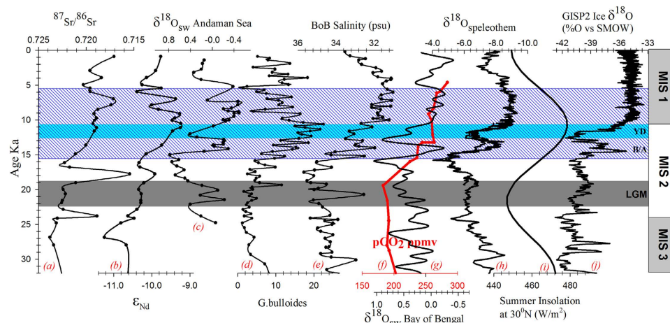
Figure 5. Downcore plots of (a) ^{87}\text{Sr}/^{86}\text{Sr} of SK168 (present study); (b) \epsilon_{\text{Nd}} of SK168 (present study); (c) \delta^{18}\text{O}_{\text{sw}} of Andaman Sea of RC12-344 29 ; (d) Planktonic foraminifer ( Globigerina Bulloides ) % in SK168 35 ; (e) Salinity record in 126KL core of Bay of Bengal 27 ; (f) \text{pCO}_2 39 ; (g) \delta^{18}\text{O}_{\text{sw}} of middle-west Bay of Bengal from SK218 28 ; (h) \delta^{18}\text{O} of stalagmites of Chinese caves 69,70 ; (i) summer insolation at 30^\circ\text{N} 31 ; (j) \delta^{18}\text{O} of ice core from Greenland ice-sheet program GISP2 71 . For clarity we have restricted the time series records to 32 ka. Descriptions for shaded region except blue can be found in Fig. 2 caption. The blue color shaded region represents the period with coeval increase in chemical weathering and the deglacial monsoon.
