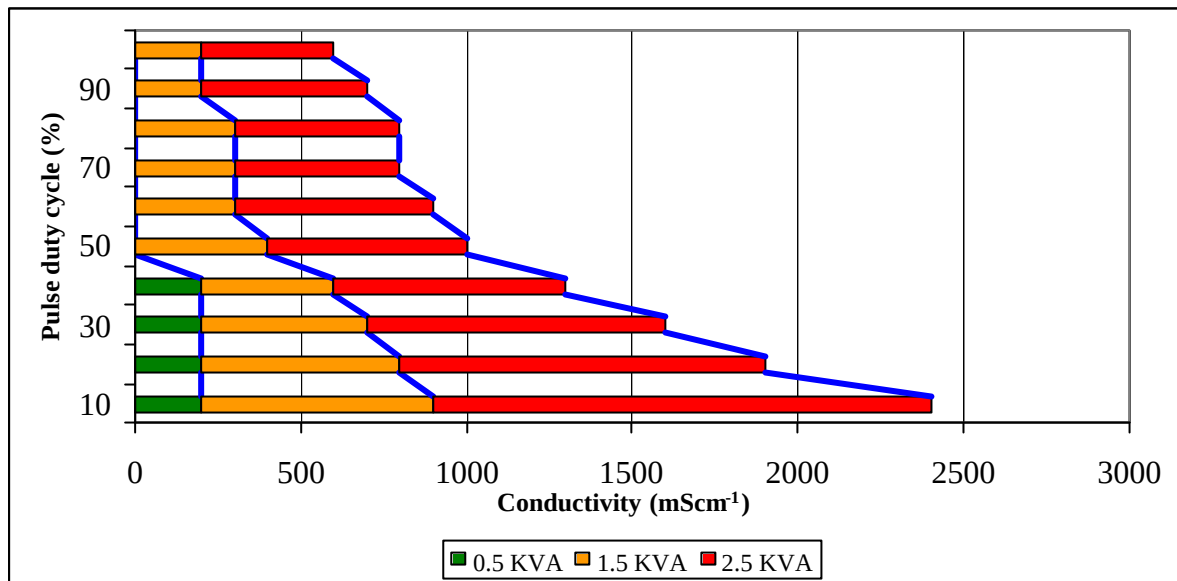
Figure 2.18 The size of generator needed to power two 400 mm anodes at different square waveform duty cycles and conductivity, at 300V, 50Hz. (note 100% duty cycle = dc)
