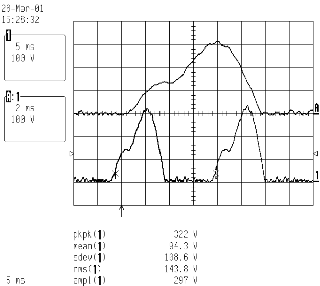
50 Hz Maximum setting 52.6Ω load PBR –V 0A
