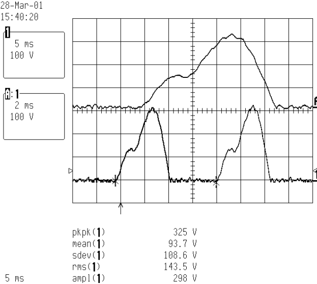
50 Hz Maximum setting 52.6Ω load PBR 230V 0A
