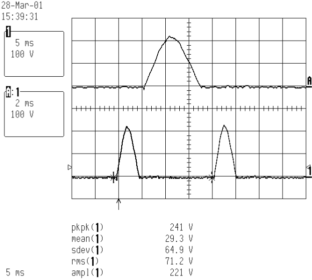
50 Hz Middle setting 52.6Ω load PBR 230V 0A
