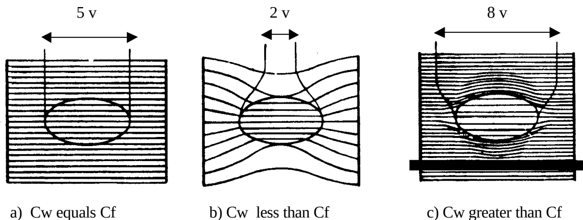
Figure 2.32 Current distribution in similar and dissimilar conductive mediums (from Brøther 1954)
