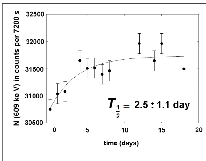
Figure 5 Count rate in the E_{\gamma}=609 keV line of ^{238}\text{U} -decay series as function of time since sealing sample #13a.
