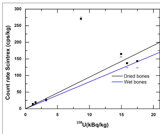
Figure 4 Count rate for wet and dry bones measured by Scintrex as function of the ^{238}\text{U} concentration, measured with HPGe detector.
