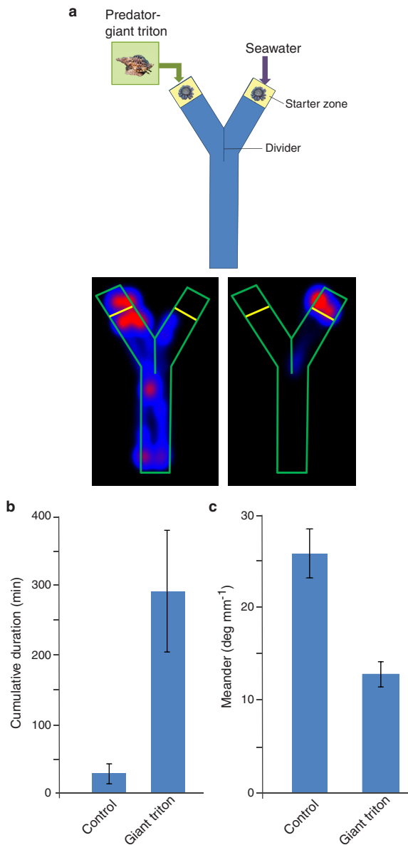
Extended Data Figure 5 | Response of crown-of-thorns starfish to seawater conditioned with its predator the giant triton, Charonia tritonis . a , Top, diagram showing Y-maze experimental design showing arm dividers and starter zones (yellow). Middle, heat maps showing the cumulative response of COTS over 45 min to water conditioned with a giant triton (left) and ambient seawater (right) ( n = 18 ). Red, area in which COTS spent most of the time with descending time to blue; black, no presence. Green outline represents the Y-maze and arm divider that prevents recirculation of water into the opposite arm; starter zones are demarcated by yellow lines. b , The duration of movement (highly active threshold set at >60\% ; t = -2.936 , P = 0.006 , 2-tailed t -test). c , The meander (change in direction of movement) of active animals over 45 min ( t = 4.437 , P = 0.000 , 2-tailed t -test). Control, ambient seawater only; giant triton, ambient seawater conditioned with giant triton exudate. Mean \pm s.e.m. See Supplementary Video 3 and Supplementary Note 7 for further details.
