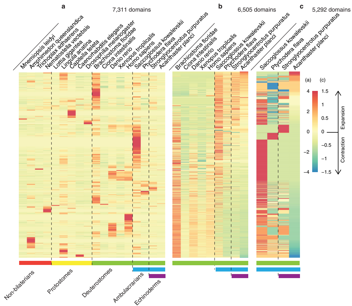
Extended Data Figure 3 | Pfam enrichment in the genomes of selected metazoans displayed as relative abundance heat maps. a , Comparison of metazoans. b , Comparison of deuterostomes. c , Comparison of ambulacrarians. See Supplementary Note 5 for further details of methods and analyses.
