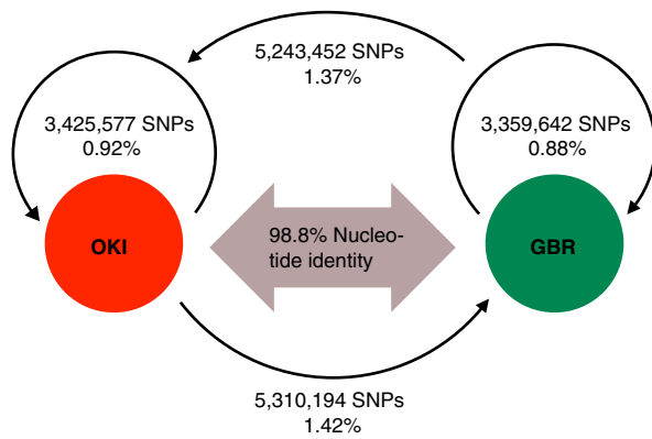
Extended Data Figure 2 | Acanthaster planci heterozygosity. a , Single-nucleotide polymorphism (SNP) analysis showing the number of SNPs identified within and between OKI and GBR genomes. Percentage heterozygosity within these genomes and the level of nucleotide variance
