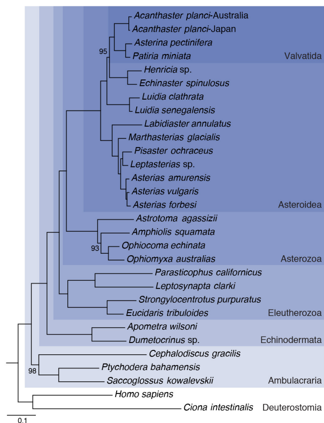
Extended Data Figure 1 | Deuterostome phylogeny showing placement of Acanthaster within asterozoa. A concatenated supermatrix of 427 genes (95,585 amino acids, 45.16% missing data) recovering a fully resolved tree. With exception of support for hemichordate monophyly (bootstrap support value = 98%), we found maximal support for all phylum- and class-level taxa. Species sampled, annotations and characteristics of each gene analysed are presented in Supplementary Note 4. Bootstrap support values below 100 are shown. Scale bar: 0.1 substitutions per site.
