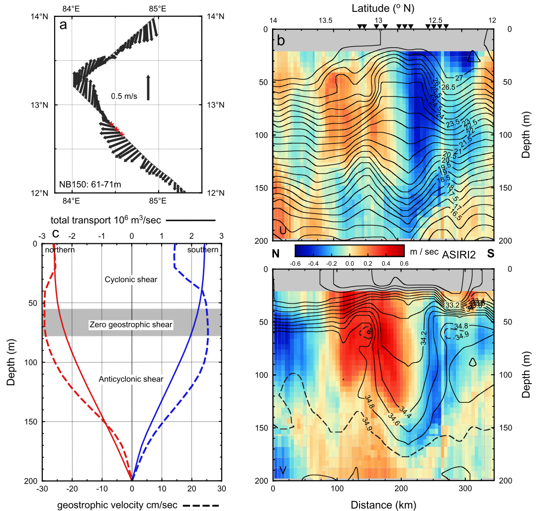
Figure 3. ITE circulation- (a) Velocity associated with the ITE from the RV Revelle ADCP within the depth interval 61–71. (b) The ADCP velocity section, the zonal component (+ is eastward) is the upper panel and meridional component (+ is northward) in the lower panel. The section is constructed from both the 75 and 150 kHz data: 75 kHz 38 m and deeper; the 150 kHz records the 21–38 m interval. Isotherms are shown on the u-component; salinity on the v-component. (c) The geostrophic velocity (dashed lines) and transport (solid lines) relative to 200 decibars, for stations to the northwest (red) and to the southeast (blue) of the ITE core. The Map was produced with GMT 4.5.2, http://gmt.soest.hawaii.edu/ .
