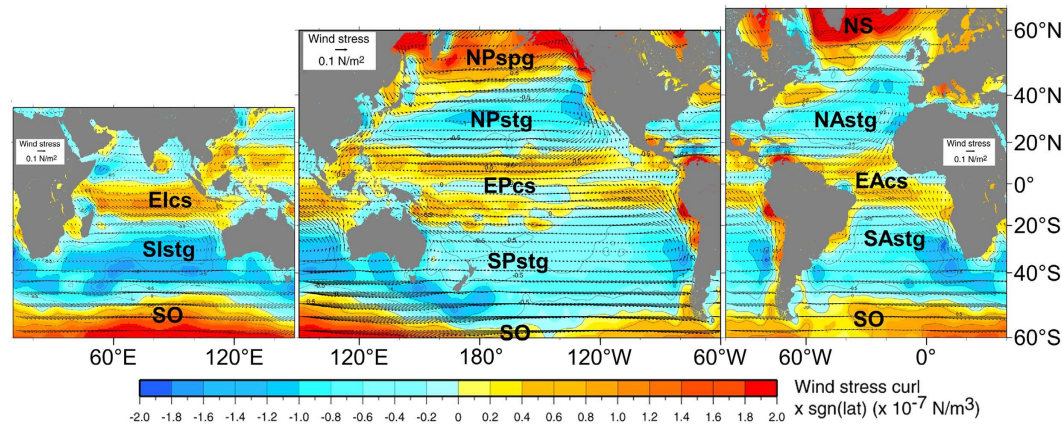
Figure 1. Surface ocean dynamics partition utilized in this work, based on the annual mean wind stress (vectors) and wind-stress curl (color shading, multiplied by -1 in the Southern Hemisphere). Based on, and modified from Figs S9.3a, S10.2a and S11.03a of the book “Descriptive physical oceanography: an introduction” by Talley et al. , Academic Press (2011) 11 , reproduced with permission. For a list of acronyms used in the figure and in the body of the paper see Table 1.
