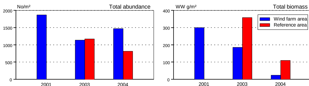
Figure 3.6. Total abundance and total biomass in the wind farm and reference areas from 2001 to 2004. Autumn samples.
