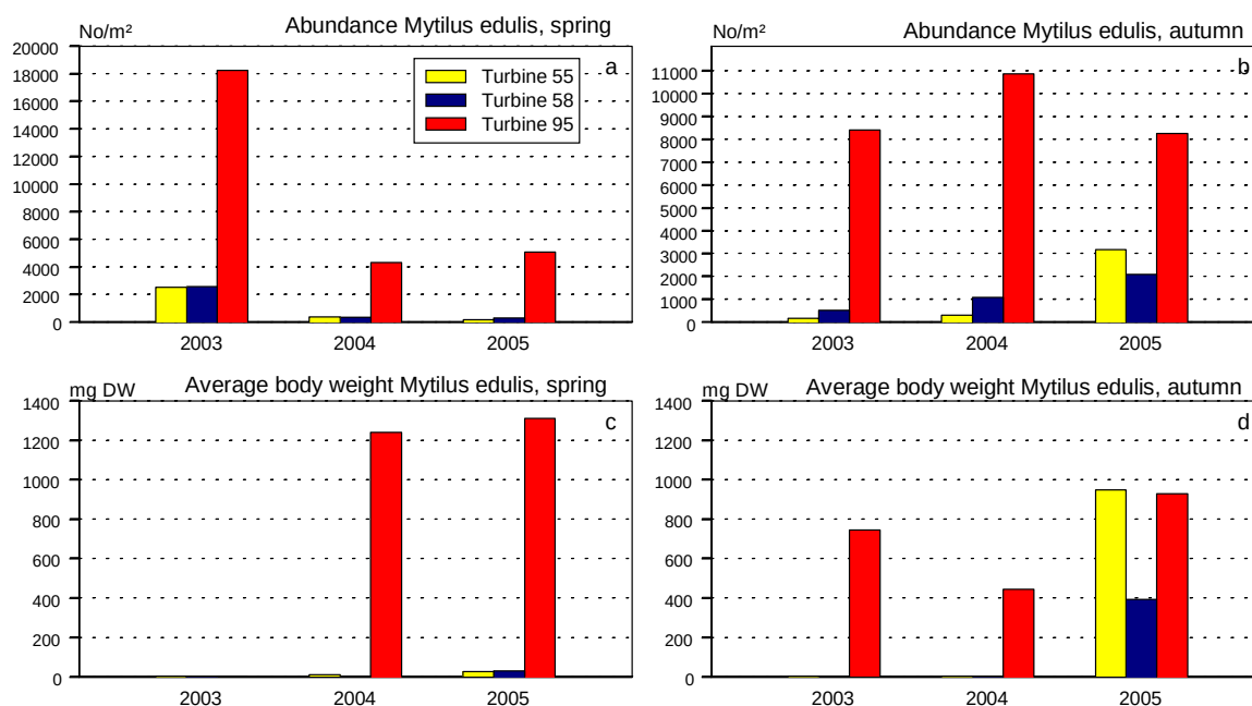
Figure 3.21. Average abundance and average body weight of Mytilus edulis at monopiles at turbine sites 55, 58 and 95.
