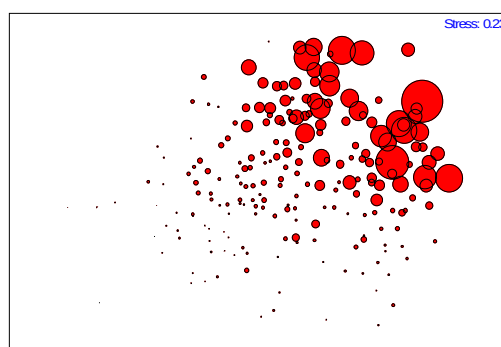
Mytilus edulis
