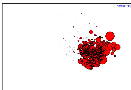
Mytilus edulis
