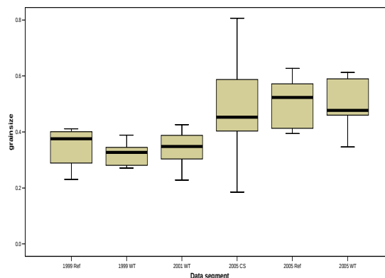
Figure 3.4. A box plot of the median grain size in the wind farm and reference areas in the spring surveys from 1999 to 2005.
