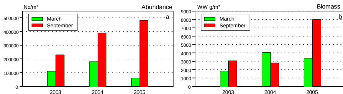
Figure 3.19. Abundance (a) and biomass (b) distribution from 2003-2005.
