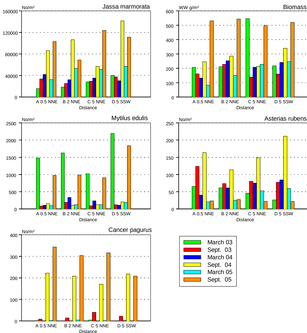
Figure 3.18. Distribution pattern on the scour protections at different distances from the monopiles shown as average abundance and average biomass.
