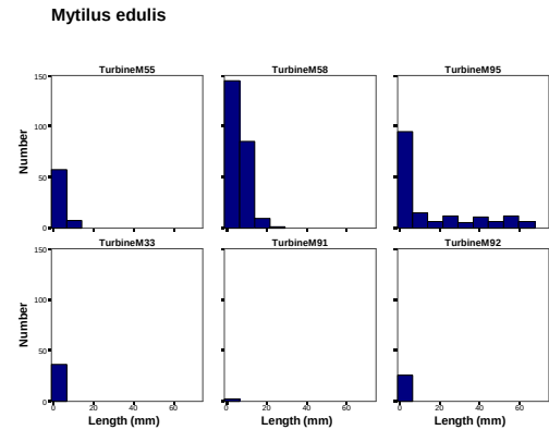
Figure 3.15.Length frequency diagram of the common mussel Mytilus edulis .
