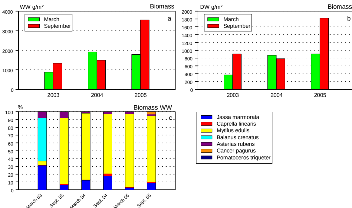
Figure 3.14. Biomass at hard bottom substrate a) Surveys wet weight. b) Surveys dry weight. c) Relative biomass of dominant species. * Differences between the wet and dry biomass distribution were mainly caused by the differences in the relative proportion between species with shells (barnacles and mussels) and without shells (amphipods).
