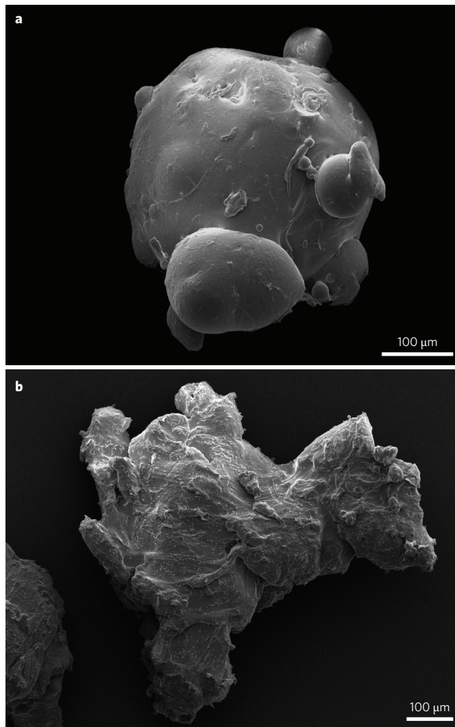
Figure 2 | Scanning electron microscopy images of microplastics.
