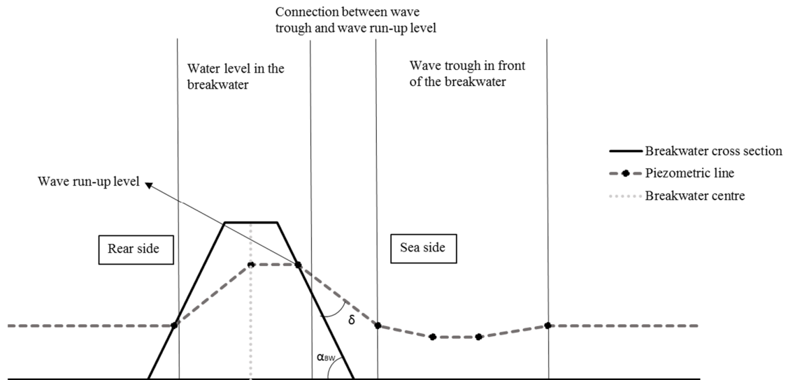
Fig. 1. An example of an applied piezometric line including a wave trough and an increased water level in the breakwater due to wave run-up
