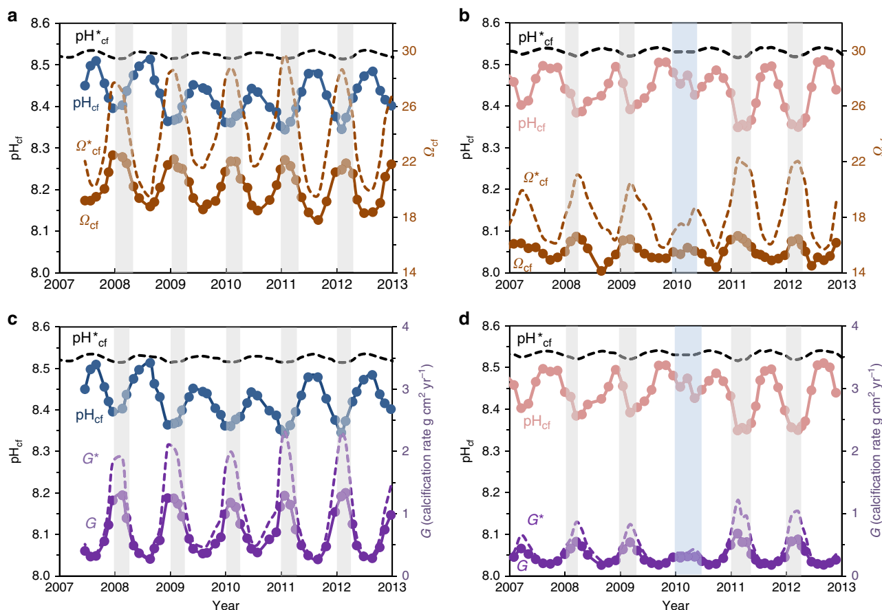
Figure 4 | Seasonal time series of calcifying fluid \text{pH}_{\text{cf}} and \Omega_{\text{cf}} together with calculated calcification rates G . (a) Calcifying fluid \text{pH}_{\text{cf}} and \Omega_{\text{cf}} values for Porites coral (D-2) from Davies Reef (GBR), where \Omega_{\text{cf}} = [\text{Ca}^{2+}]_{\text{cf}} [\text{CO}_3^{2-}]_{\text{cf}} / K_{\text{arag}} . Dashed line shows the \Omega_{\text{cf}}^* calculated using fixed experimental 10,17 \text{pH}_{\text{cf}}^* values (see Fig. 2a,b). (b) Same as previous for Coral Bay (Ningaloo Reef, Western Australia) Porites (CB-2). (c) Calcification rates calculated using the inorganic rate equation 28 G = k(\Omega - 1)^n , where k and n are the temperature-dependent constant and order of the reaction, respectively 28 . Because of opposing changes in \text{pH}_{\text{cf}} relative to \text{DIC}_{\text{cf}} (Fig. 1), \Omega_{\text{cf}} and hence coral growth rates are strongly modulated reducing seasonal variations by twofold compared to those estimated from fixed condition experiments ( G^* ). (d) Same as previous for Porites from Coral Bay (Ningaloo Reef, Western Australia).
