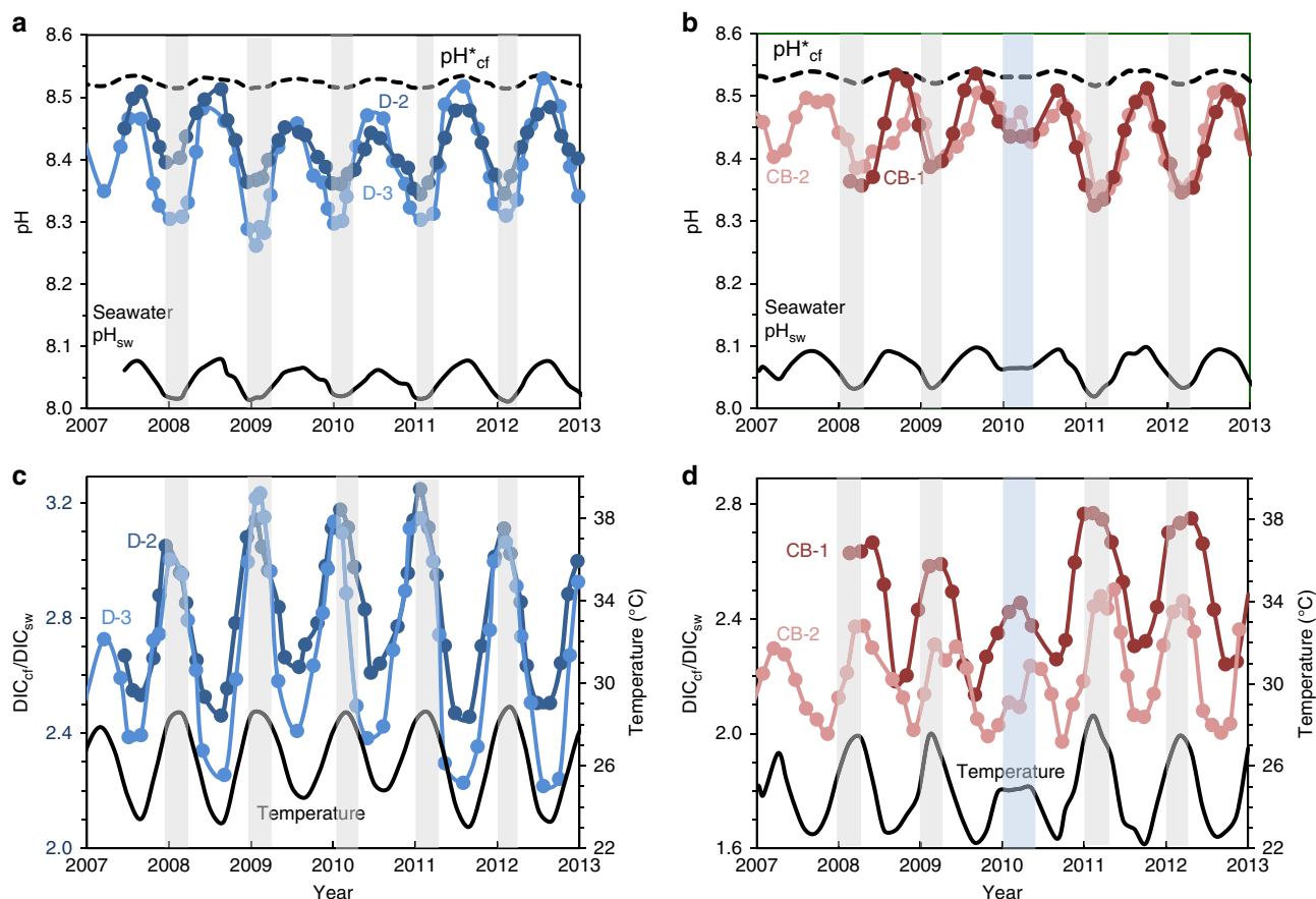
Figure 2 | Seasonal time series of coral calcifying fluid pH cf and DIC cf . (a) Porites spp. coral calcifying fluid pH cf derived from \delta^{11}\text{B} systematics (see 'Methods' section and Supplementary Data) for colonies D-2 and D-3 from Davies Reef (18.8° S) in the Great Barrier Reef, Queensland. Shading denotes the summer period when pH cf and seawater pH sw values are at a minimum. Dashed line shows pH cf expected from artificial experimental calibrations ( \text{pH}_{\text{cf}}^* = 0.32 \text{ pH}_{\text{sw}} + 5.2 ) 10,17 with an order of magnitude lower seasonal range than measured pH cf values. (b) Same as previous for Porites colonies from Coral Bay (CB-1 and CB-2) in the Ningaloo Reef of Western Australia (23.2° S) showing seasonal fluctuations in pH cf and seawater pH sw . The blue shading denotes the anomalously cool summer temperatures in 2010. (c) Enrichments in calcifying fluid DIC cf (left axis; coloured circles) derived from combined B/Ca and \delta^{11}\text{B} systematics together with synchronous seasonal variations in reef-water temperatures (right axis; black line) for Porites colonies from Davies Reef (GBR). The strong temperature/light control on DIC cf is consistent with enhanced metabolic activity of zooxanthellae symbionts in summer. (d) Same as previous but for Porites from Coral Bay (Ningaloo Reef, Western Australia).
