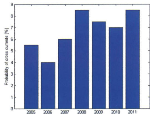
Figure 17: Evolution in the predicted probability of cross currents.
