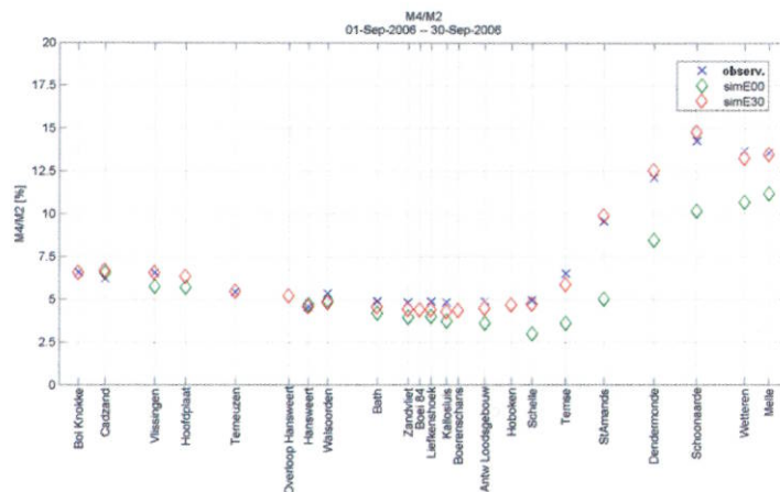
Figure 11: Improvement of the M4/M2 tidal asymmetry (%) along the entire estuary. SimE00 is before and SimE30 is after recalibration of the model.
