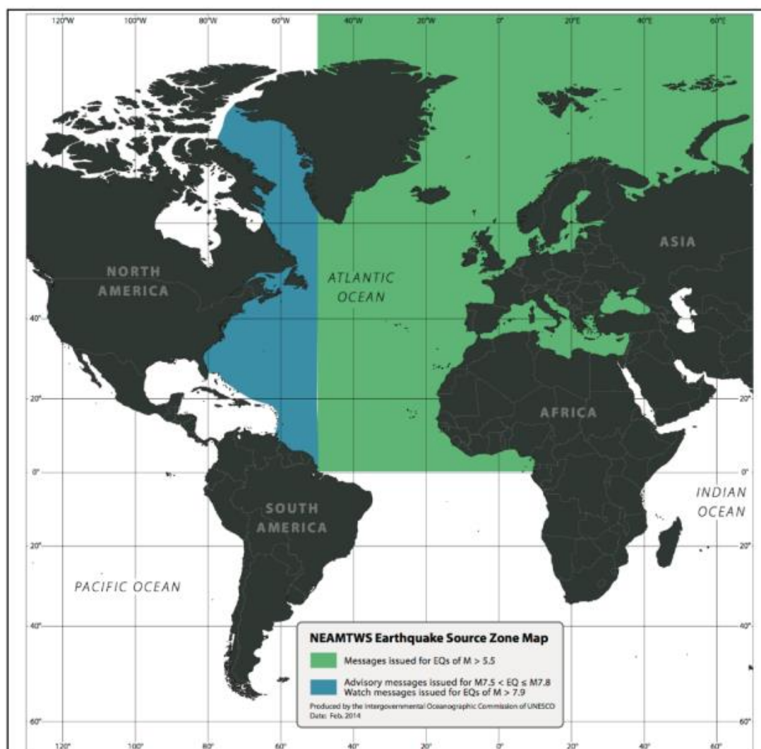
Figure: NEAMTWS Earthquake Source Zone Map (Reference: IOC/TOWS-WG-VIII/3 Annex V, page 21)
