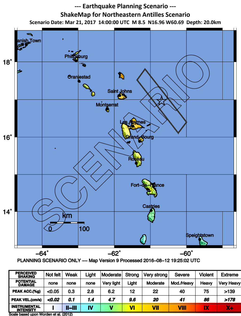
Figure D5. Shake map output for the CARIBE WAVE 17 Northeastern Antilles earthquake scenario.
