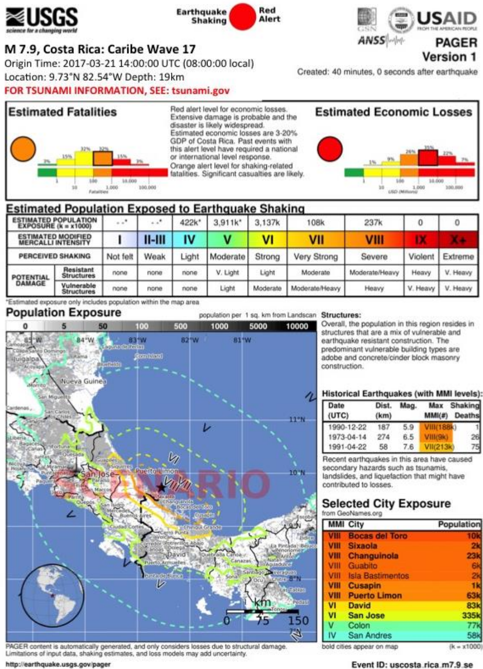
Figure D2. PAGER output for CARIBE WAVE 17 Costa Rica earthquake scenario (USGS).
