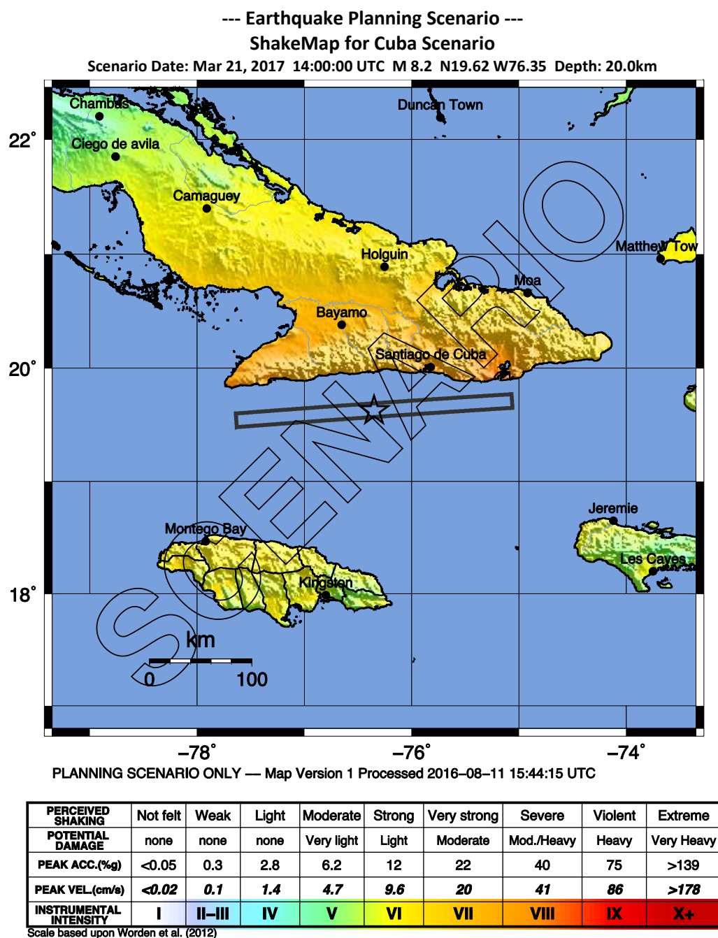
Figure D3. Shake map output for the CARIBE WAVE 17 Cuba earthquake scenario.
