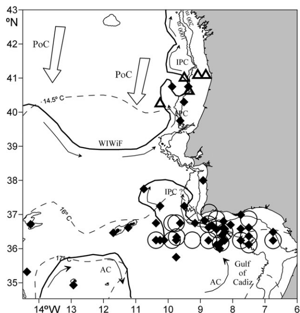
Fig. 12. Distribution of paralarvae of oceanic species. Open triangles are the Teuthowenia megalops records, open circles are the tropical/sub-tropical species ( Abralia cf. veranyi , Ancistrocheirus lesueurii , Pyroteuthis margaritifera , Helicocranchia pfefferi , Megalocranchia sp. and Leachia sp.) and dots represent the remaining species distribution. Overlay of winter sea surface temperature (SST) and major winter surface circulation features, after Peliz et al. (Peliz et al. , 2005): PoC, Portugal Current; IPC, Iberian Poleward Current; AC, Azores current eastern branch (arrows); WiWiF, Western Iberia Winter front, Gulf of Cadiz northern re-circulation and STF/AC frontal systems (thick lines).
