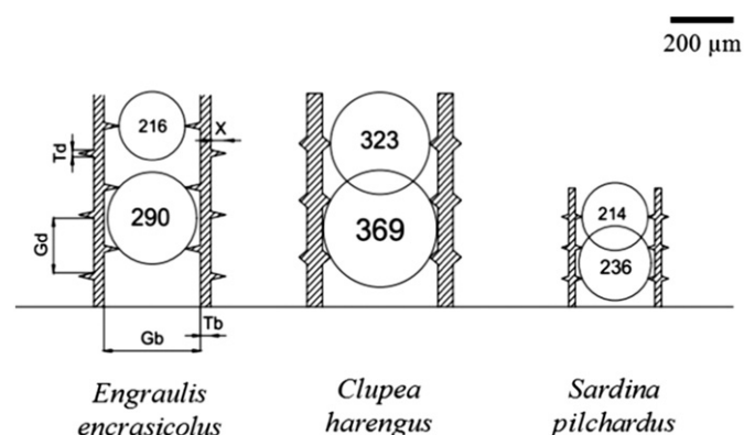
Fig. 6. Diagrams showing the minimum diameter of particles retained in the three species. Gb: gap between GRs; Gd: gap between denticles; Tb: GR thickness; Td: denticle thickness; X: denticle length. Modified from Gibson (1988).
