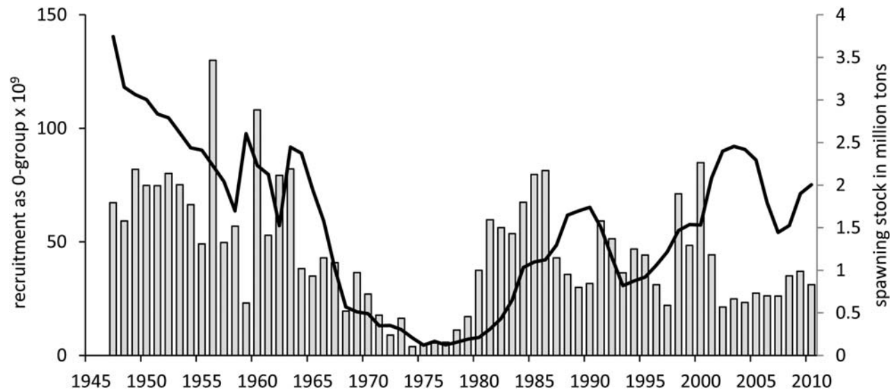
Figure 1. Spawning stock (drawn line) and recruitment produced by that stock (bars) for North Sea herring. Data from ICES (2012).
