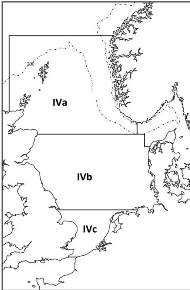
Figure 12. ICES North Sea Divisions referred to in Figure 11.
