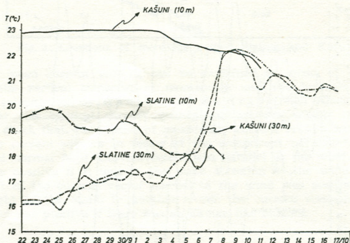
Fig. 3: Time-series of daily mean temperature for two moorings. Strong temperature increase at the depth of 30 meters coincides with the start of the SE-wind.
