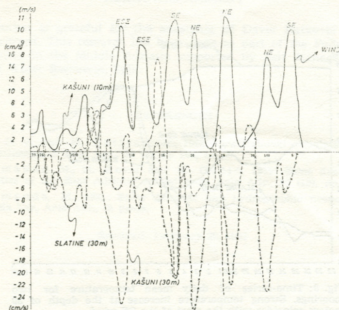
Fig. 2: Time-series of wind speed and wind-ward current component. Positive current component is in the direction of the wind, while the negative one is in the opposite direction.
