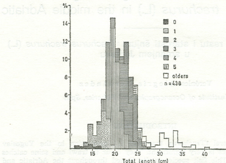
Fig. 1. Length frequency and age distribution of sampled Trachurus trachurus (L.) from Blitvenica in the Adriatic Sea in 1980—1981.
