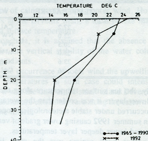
Fig. 2. Average vertical temperature distribution in August at permanent station Kaštela Bay (collected in the period 1965-1990) and values for August 1992
