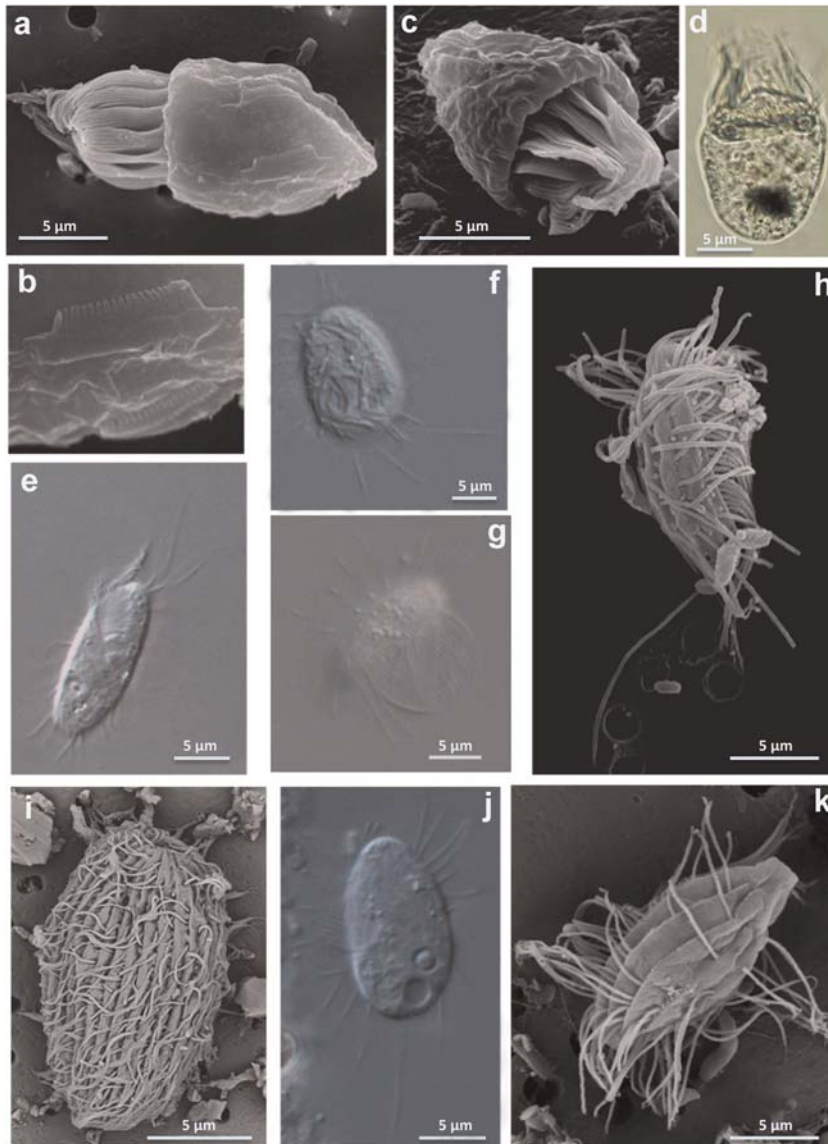
Fig. 5. Some species of nanociliates detected in this study. (a–c) Strobilidium sp. with distinct somatic kinety rows (b) SEM, \times 7000 , \times 12\,000 and \times 14\,000 , respectively. (d) Rimostrombidium humile , BF, \times 1350 . (e) Cyrtolophosis mucicola , DIC, \times 1350 . (f) Cinetochilum margaritaceum , DIC, \times 1350 . (g) Cyclidium candens , DIC, \times 1350 . (h) Cyclidium sp., SEM, \times 5000 . (i) Unidentified prostome ciliate, SEM, \times 5000 . (j) Cyclidium glaucoma , DIC, \times 1350 . (k) Cyclidium sp., SEM, \times 5000 . Bar represents 5 \mu\text{m} .
