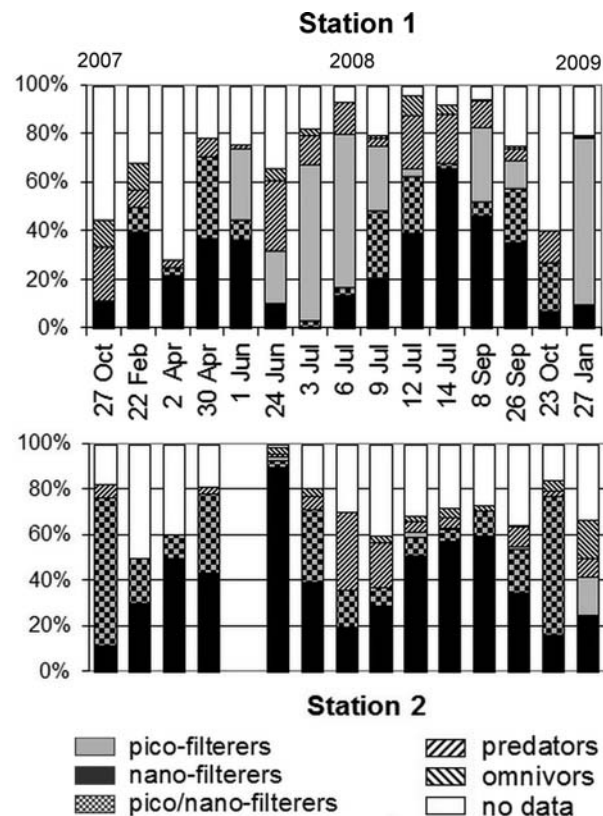
Fig. 7. Seasonal dynamics of abundance (percentage) of ciliates from different trophic groups; pico-filterers (bactivoracious), nano-filterers (algivorous + consumers of heterotrophic flagellates + mixotrophic), pico-/nano-filterers (bacterio/algivorous), predators (feeding on ciliates), omnivores (feeding on algae, heterotrophic flagellates and ciliates). Myrionecta rubra excluded (<3.5% of total abundance). Top panel: Station 1; bottom panel: Station 2.
