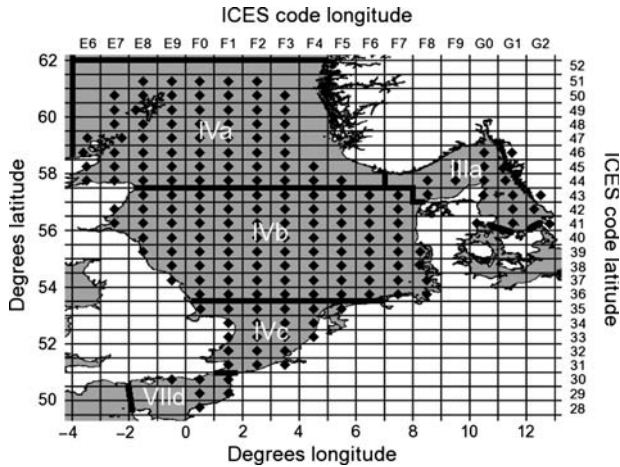
Figure 1. Map showing the area sampled by the IBTS during the first quarter of years 1986–2011. The bold lines delineate ICES Subareas, labelled as IIIa, IVa, IVb, IVc and VIId (ICES, 1977; http://www.fao.org/fishery/area/Area27/en ). ICES rectangles marked with a diamond have at least one fish sampled by the IBTS during 1986–2011, according to DATRAS. This figure is based on ERSI shape files downloaded from ICES ( http://geo.ices.dk/ ). Detailed maps of IBTS-sampled rectangles by year and species are available directly from ICES ( http://ecosystemdata.ices.dk/Map/ ).
