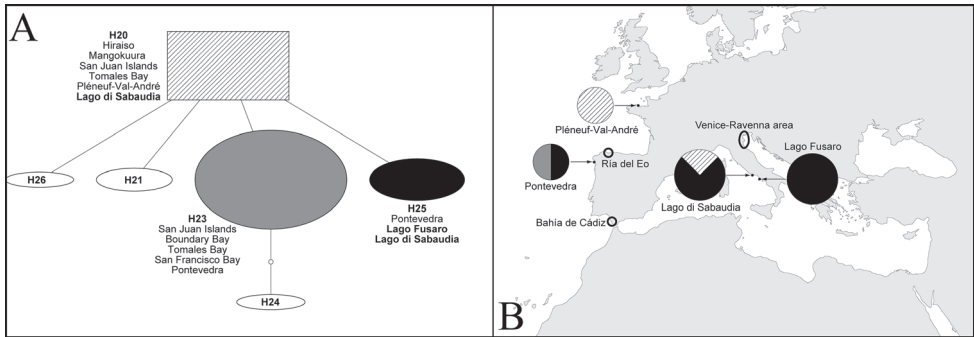
Figure 2. A. Haplotype network of non-native haplotypes of Haminoea japonica Pilsbry, 1895 (haplotype IDs from Hanson et al. 2013). Rectangular haplotype (H20) is most ancestral. Sizes of the haplotype icons are proportional to the total number of individuals sequenced (data from Hanson et al. 2013 and present paper). B. Known European records of H. japonica , including new collection localities. Sizes of the pie charts are proportional to the number of individuals sequenced from the locality. Pie charts and patterns within indicate the proportion of different haplotypes found in each locality.
