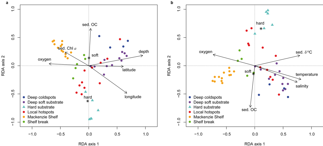
Figure 7. Redundancy analysis (RDA) ordination plots of megabenthic biomass-based taxonomic composition against forward selected environmental variables (black arrows and centroids) on 50 stations from 2008 to 2011. (a) Including indirect/spatial variables; the first two RDA axes explained 61% of the variance. (b) Without spatial variables; the first two RDA axes explained 64% of the variance. The categorical variable ‘substrate type’ is illustrated using centroids (*) for each category (hard and soft) and colors represent the six benthic communities defined in this study. doi:10.1371/journal.pone.0100900.g007
