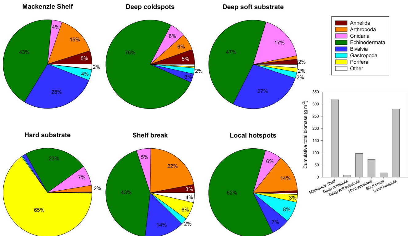
Figure 6. Variation in mean relative biomass composition (%) (only ≥2% shown) for the main phyla or classes sampled in all community clusters (pie charts) and cumulative total biomass ( \text{g m}^{-2} ) sampled per community cluster (histogram). doi:10.1371/journal.pone.0100900.g006
