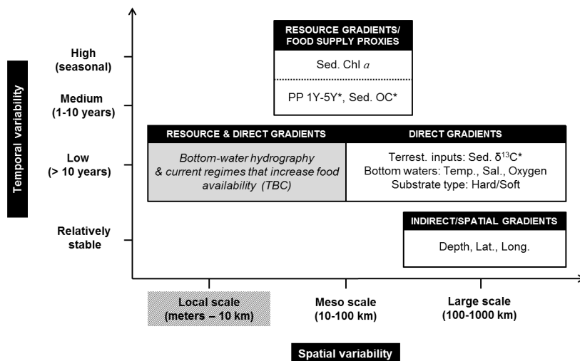
Figure 8. Conceptual figure displaying the overall results of environmental drivers of megabenthic communities in this study in relation to their spatial and temporal scales of variability; potential missing important drivers (gray box) would have to be confirmed (TBC). Environmental factors available for the present study were divided into three categories: resource, direct and indirect/spatial gradients (following [14]). Sampling design of the present study prevented conclusion at local scale (dashed). * denotes environmental variables that were either significantly correlated with univariate community characteristics or to community cluster distribution. doi:10.1371/journal.pone.0100900.g008
