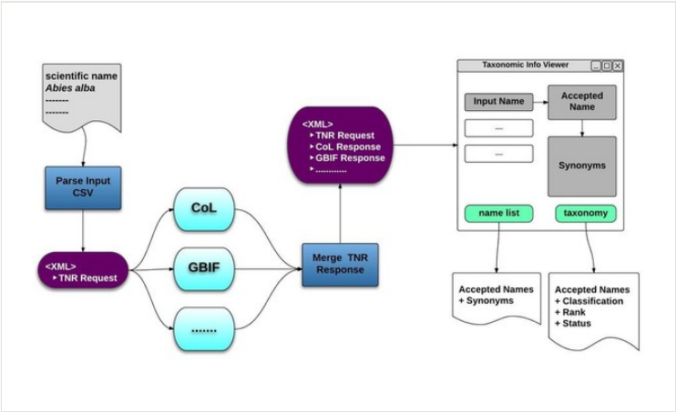
Figure 2. Taxonomic Name Resolution. Overview of the Name Resolution function of the Taxonomic Data Refinement Workflow, depicting the aggregation of scientific name responses from the various checklist into a single XML message. This message is then used to display the results within a web interface.
