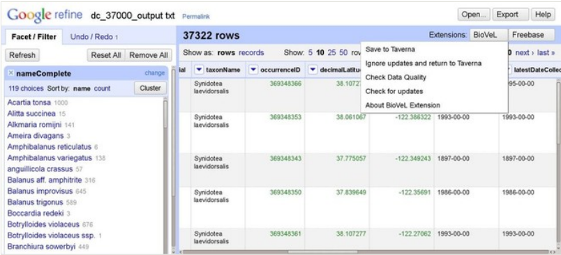
Figure 3. OpenRefine interface with the BioVeL extension. The extension adds biodiversity data specific functionality to OpenRefine for the purposes of data cleaning, integration, and refinement. The GoogleRefine branding in the screenshot is due to the fact this workflow uses the last stable released version (2.5) of OpenRefine when the software was still being developed by Google.
