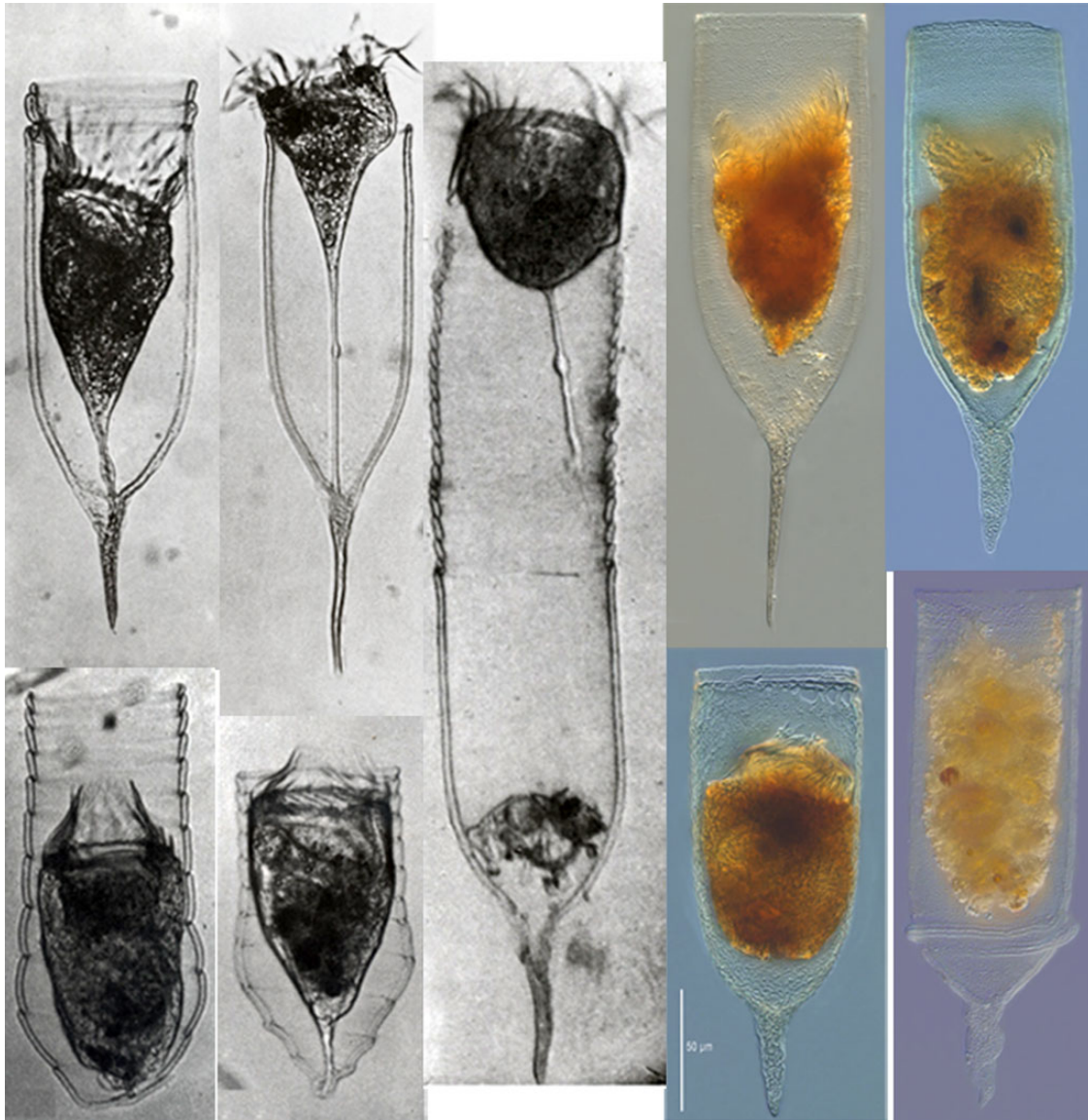
Fig. 2. Variability of F. ehrenbergii in culture and a natural population. Left and center image are bright field photomicrographs of the different loricas formed in culture [adapted from Laval-Peuto (Laval-Peuto, 1983), with permission of author/copyright holder]. Right side images are differential interference contrast photomicrographs of cells from a natural population in a mesocosm experiment, original micrographs.
