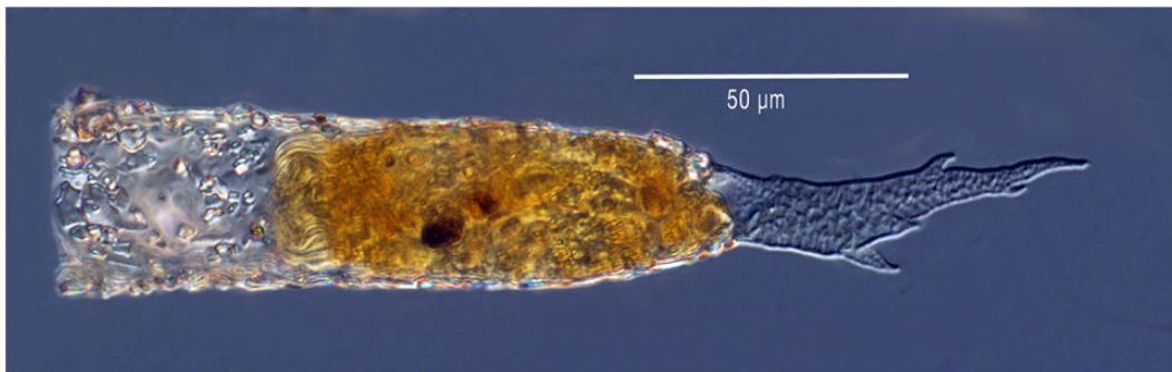
Fig. 1. The species now known as R. tagatzi described by Strelkow and Wirketis (Strelkow and Wirketis, 1950), formerly described as a variety of T. karajensis (Busch, 1925), as well as T. corniger (Hada, 1964) and T. nudicauda (Paulmier, 1997). Specimen from S te, France, on the Northwest coast of the Mediterranean Sea, original micrograph.
