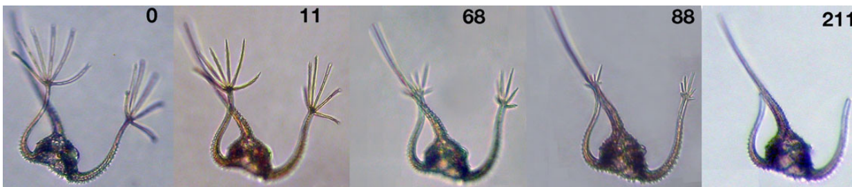
Fig. 3. The dinoflagellate C. ranipes absorbs its “fingers” at night. Images are of the same individual photographed at intervals from the beginning of the dark period, 0, to after 211 min of darkness. Absorption of the fingers takes about 2 h, fingers are re-formed at the beginning of the light period. Adapted from Pizay et al. (Pizay et al. , 2009), with permission of Elsevier.
