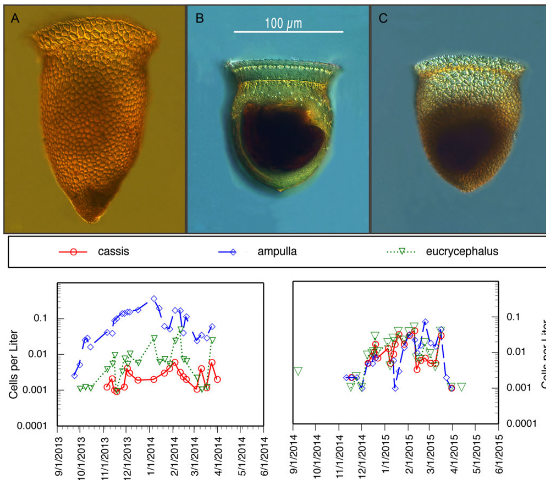
Fig. 4. The three most common morphs of C. ampulla : cassis (A), ampulla (B), eucrycephalus (C) and their abundance in the Bay of Villefranche in autumn–winter of 2013–2014 and autumn–winter of 2014–2015. From the beginning of September to the end of May, for each date material from the equivalent of 500 L (plankton net tow 0–75 m) was examined yielding a detection limit of 0.002 cells per liter averaged over 0–75 m. Original micrographs.
