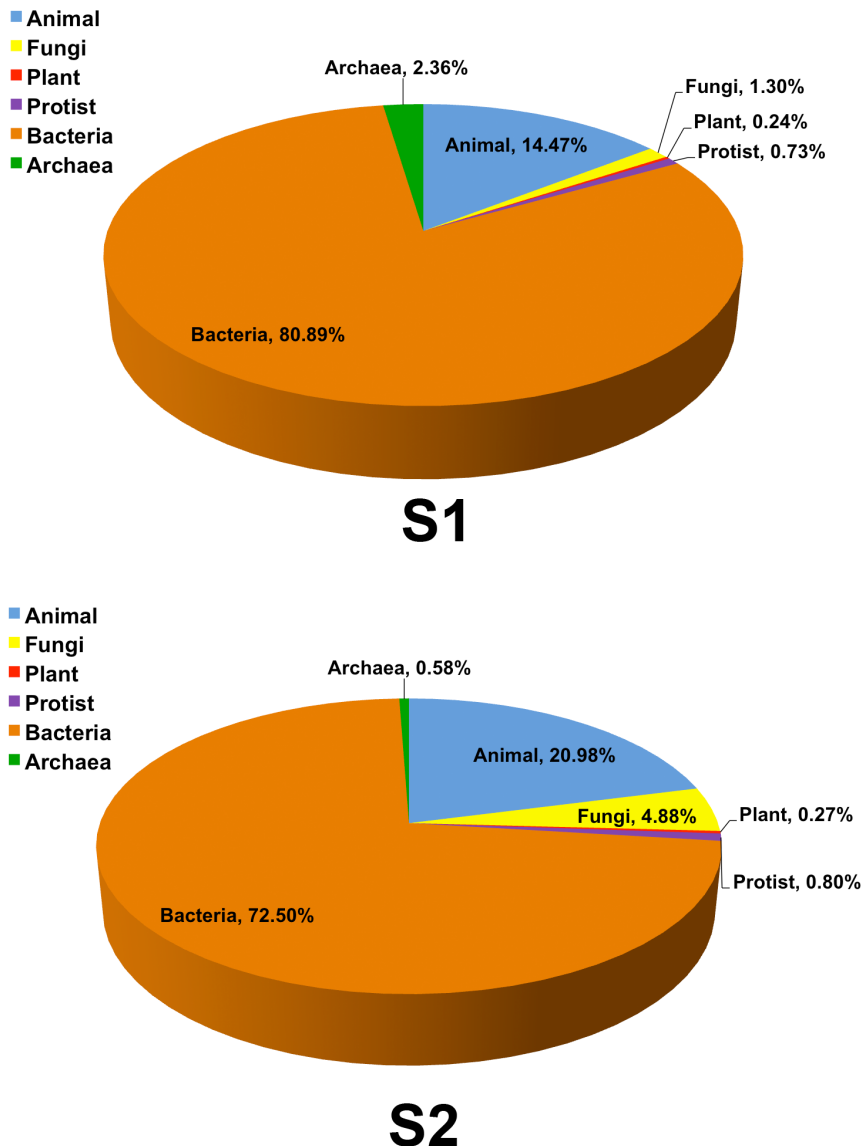
Figure 3. Percentages of 6 kingdoms of lives in S 1 and S 2 . doi:10.1371/journal.pone.0094236.g003
