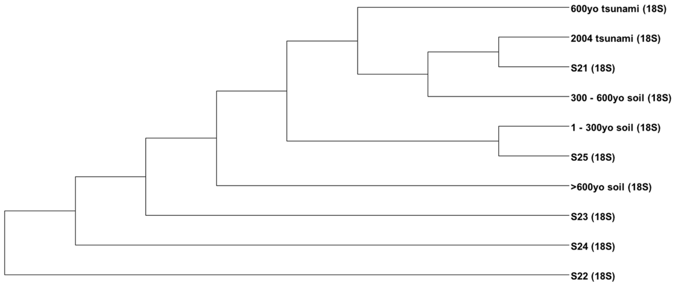
Figure 6. UPGMA clustering comparing relatedness among S_1 and S_2 prokaryotic (A) and eukaryotic (B) profiles.
