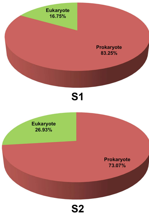
Figure 2. Percentages of prokaryotic and eukaryotic domains in S 1 and S 2 . doi:10.1371/journal.pone.0094236.g002
