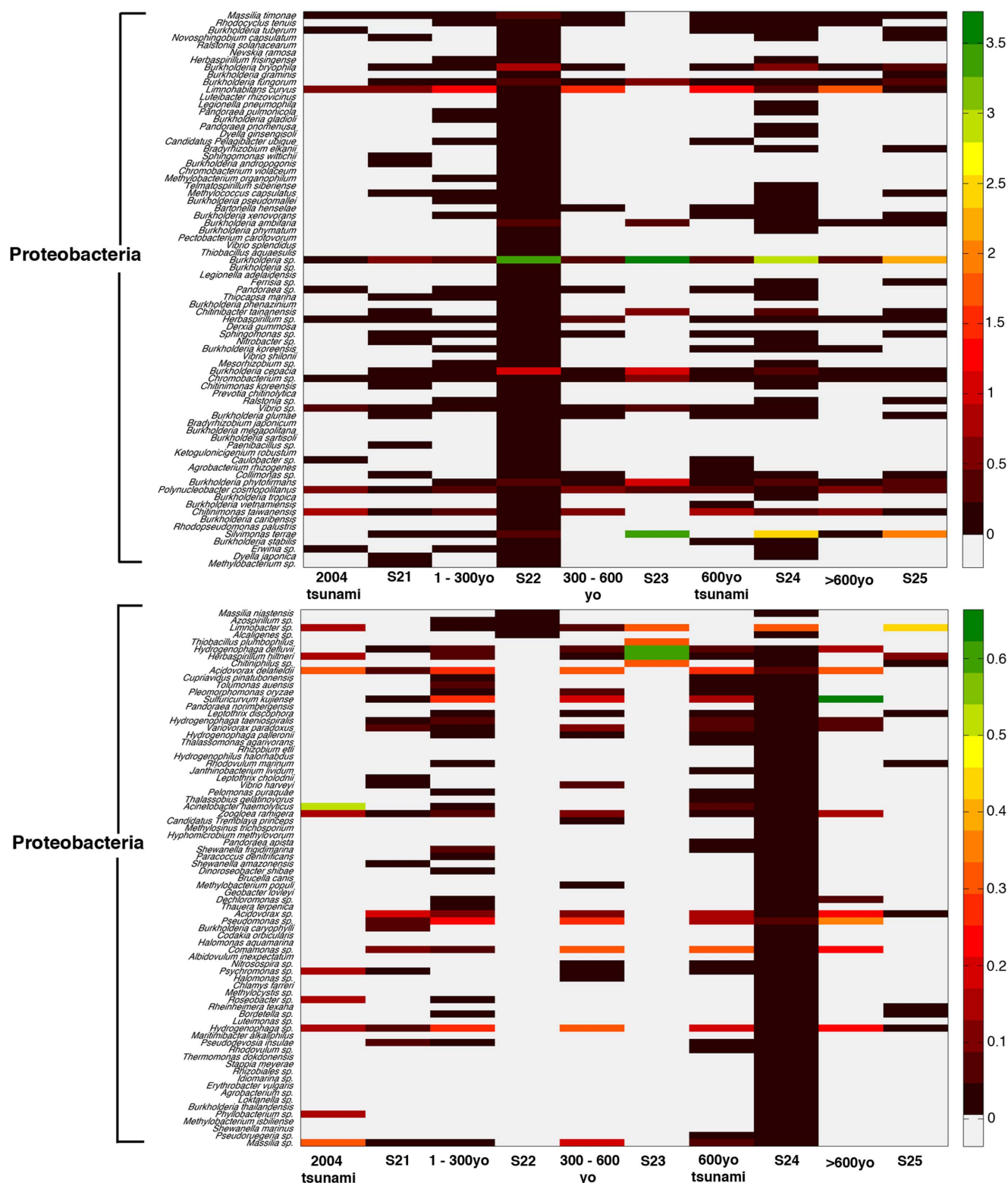
Figure 5. Distribution of prokaryotic species in S 1 and S 2 , categorized by individual sample ages. Different color on the diagram represents a different relative abundance, based on the percent frequency chart on the right. doi:10.1371/journal.pone.0094236.g005
