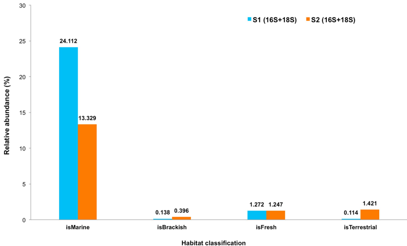
Figure 10. Habitat classification for S 1 and S 2 . Prokaryotic and eukaryotic species profiles of S 1 and S 2 were matched against WoRMS database for habitat classification.
