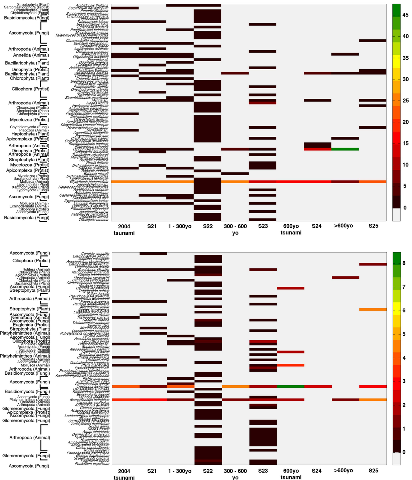
Figure 9. Distribution of eukaryotic species in S 1 and S 2 , categorized by individual sample ages. Different color on the diagram represents a different relative abundance, based on the percent frequency chart on the right. doi:10.1371/journal.pone.0094236.g009
