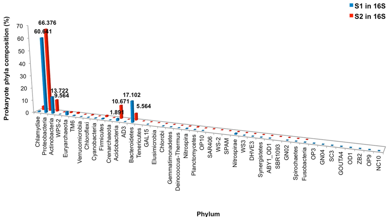
Figure 4. Distribution of prokaryotic phyla in S 1 and S 2 , without (A) and with (B) individual sample ages categorization. doi:10.1371/journal.pone.0094236.g004
