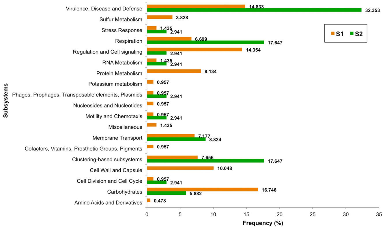
Figure 7. Metabolic subsystems of prokaryotic communities in S 1 and S 2 . doi:10.1371/journal.pone.0094236.g007
