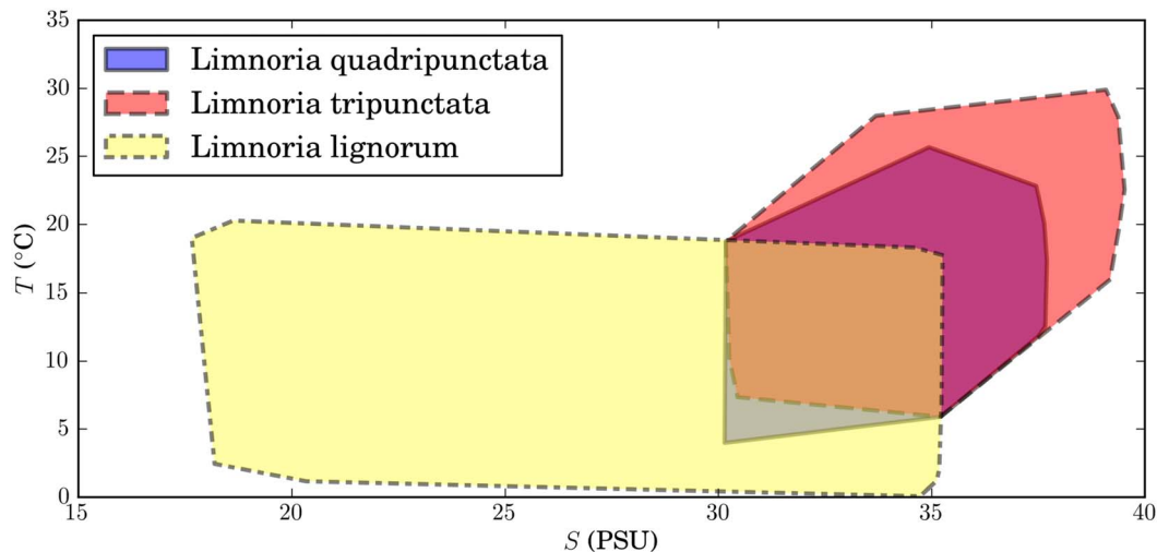
Figure 4. Distribution of the three limnoriid species in salinity-temperature ( S - T ) space. The minimum convex polygon encompassing all data points represent the climatic niche of each species. doi:10.1371/journal.pone.0109593.g004
