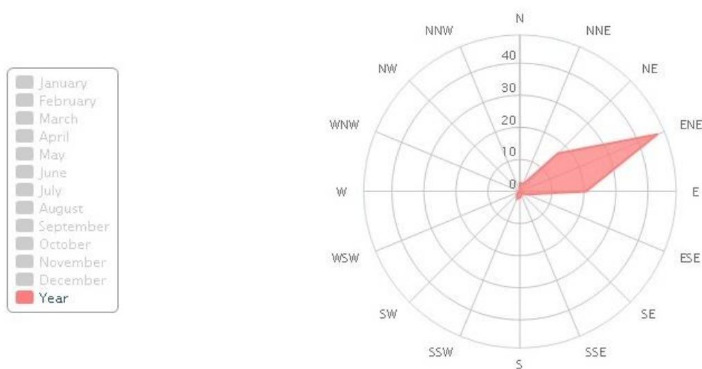
Fig. 6 Wind statistics of St-Eustatius: http://www.windfinder.com/windstatistics/st_eustatius
