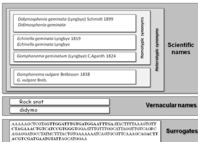
Fig 2. Reconciliation of alternative names for the same taxon (an invasive diatom species). The diagram shows three classes of ‘names’ that act in the same way as names (sequence data in this example). Gomphonema vulgare and Echinella geminata were applied independently to the same species and are heterotypic synonyms. The reconciliation group includes the homotypic synonyms ( Echinella geminata and Didymosphenia geminata ), and the lexical variants of all names. Reconciliation groups allow computer-based queries initiated with one name to be answered with information associated with all names.
