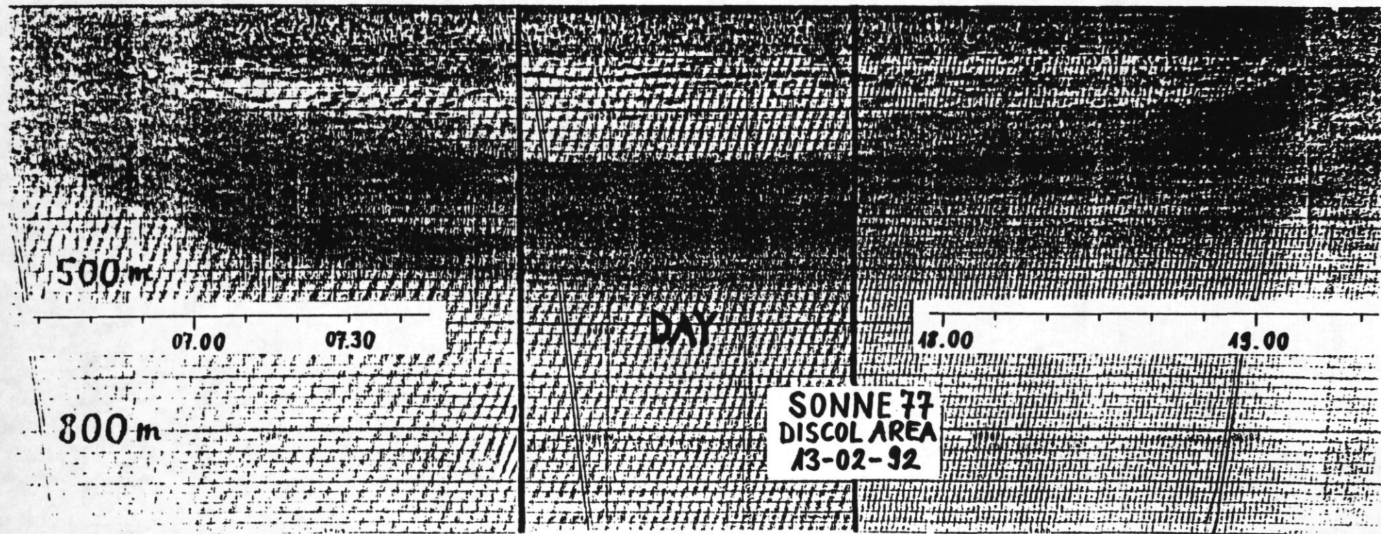
Figure 15: The Deep Scattering Layer (DSL) in the DISCOL area during SONNE 77, February 1992.
