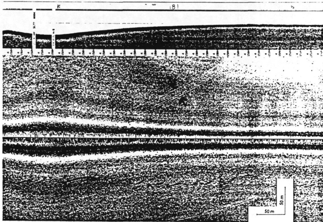
Figure 20: Side-scan sonar record of 16m wide plow-harrow track
