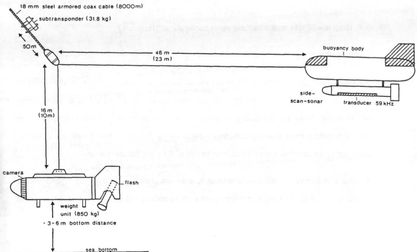
Figure 11: The side-scan sonar equipment
