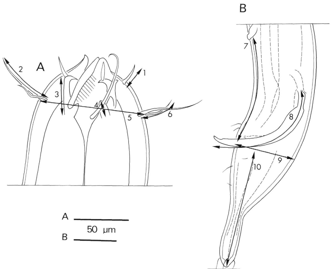
Fig. 1. - Distances measured on cameria lucida drawings of the pharynx (A) and anal (B) regions of Enoploides stewarti . 1. Inner labial seta; 2. Outer labial seta; 3. Mandible height; 4. Onchium length; 5. Head width; 6. Cephalic seta; 7. Anus to Supplement distance; 8. Spicule arc length; 9. Width at Anus; 10. Tail length.
