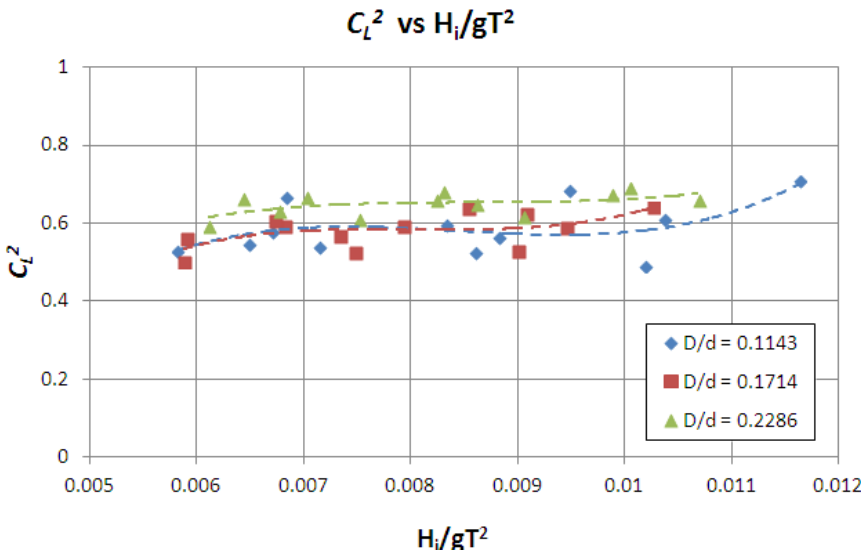
Figure 6: Energy loss coefficient C_L .
