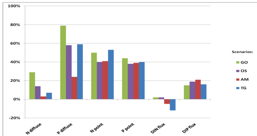
Figure 14 Expected changes in diffuse emissions of Nitrogen and Phosphorus (N diffuse and P diffuse respectively), in point emissions of Nitrogen and Phosphorus (N point and P point respectively) and in the fluxes of Dissolved Inorganic Nitrogen and Dissolved Inorganic Phosphorus (DIN flux and DIP flux respectively) in the Mediterranean Sea by the year 2030, according to the four different MEA scenarios.
