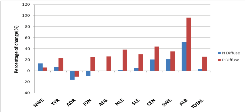
Figure 17 Expected changes in diffuse emissions of Nitrogen and Phosphorus (N diffuse and P diffuse respectively) by the year 2030, according to the Adapting Mosaic (AM) scenario, in the different Mediterranean sub-basins*.
