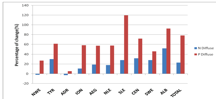
Figure 15 Expected changes in diffuse emissions of Nitrogen and Phosphorus (N diffuse and P diffuse respectively) by the year 2030, according to the Global Orchestration (GO) scenario, in the different Mediterranean sub-basins*.
