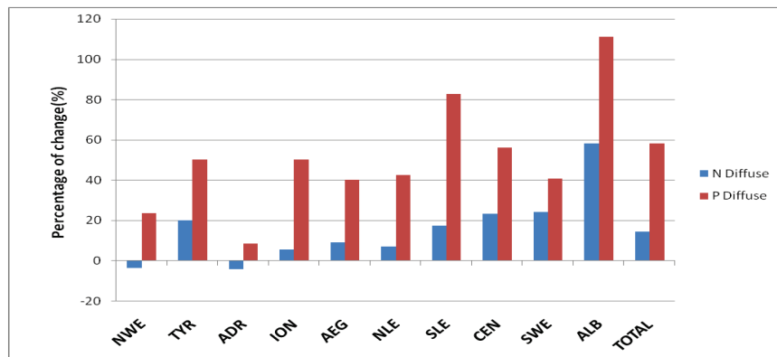
Figure 16 Expected changes in diffuse emissions of Nitrogen and Phosphorus (N diffuse and P diffuse respectively) by the year 2030, according to the Order from Strength (OS) scenario, in the different Mediterranean sub-basins*.
