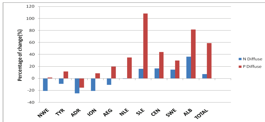
Figure 18 Expected changes in diffuse emissions of Nitrogen and Phosphorus (N diffuse and P diffuse respectively) by the year 2030, according to the Technogarden (TG) scenario, in the different Mediterranean sub-basins*.
