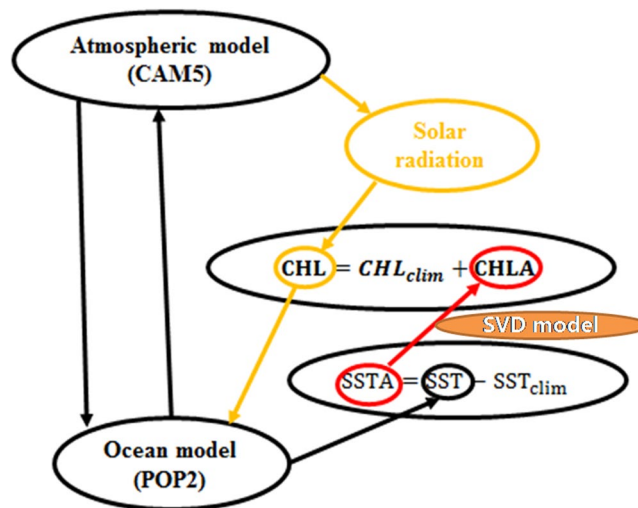
Figure 1. A schematic diagram illustrating the inclusion of the CHL-induced bio-feedback using the NCAR CESM, consisting of the original atmosphere model (CAM5) and the OGCM (POP2), and an embedded statistical representation for interannual CHL variability developed in this work. The total CHL field is separated into its climatological component ( CHL_{clim} ) and interannual anomaly component ( CHL_{inter} ), written as CHL = CHL_{clim} + CHL_{inter} which directly affect the vertical distribution of the incoming solar radiation in the upper ocean. The statistical relationships between the interannual variations in SST and CHL are derived from satellite observations and used to explicitly calculate CHLAs in the CESM to represent CHL-induced heating effects.
