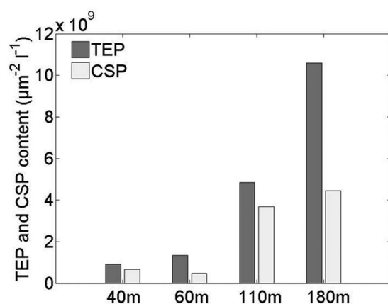
Figure 3. Content of transparent expolymers (TEP) and Coomassie Stainable Particles (CSP) at day 6 in \mu\text{m}^{-2} \text{l}^{-1} in the different depth treatments.
