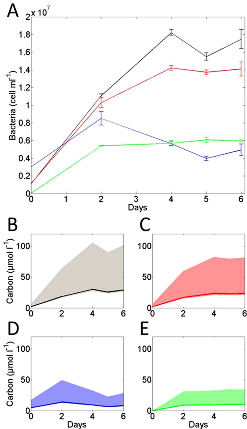
Figure 4. (A) Abundance of bacteria ( \text{cell ml}^{-1} ) and associated standard deviation from duplicates. Black line represents 40 m samples; red, 60 m; blue, 110 m and green, 180 m. The estimated equivalent in carbon ( \mu\text{mol l}^{-1} ) is presented in (B) for 40 m, (C) for 60 m, (D) for 110 m and (E) for 180 m. The bold line represents estimates following cell biomass conversion factor 42 , the shaded area around the line represents for lower and upper values using lower and values for the cell biomass conversion factor as described in ref. 41 . See text for more detailed information.
