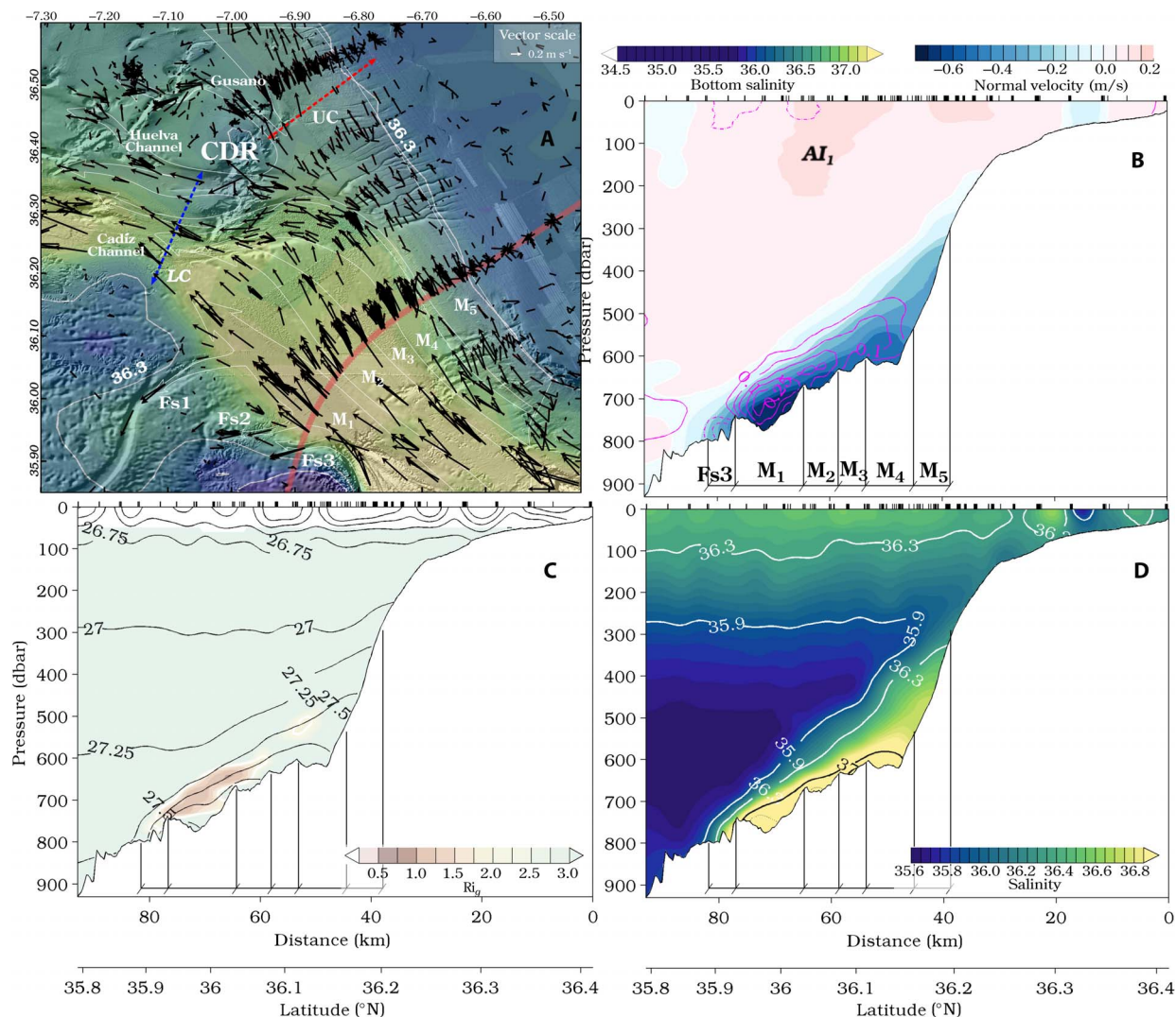
Fig. 5. Consolidated MOW branches. (A). Inset 3 of Fig. 1C. The CDR and the Gusano, Cadiz, and Huelva channels are labeled. Fs1 to Fs3 indicate the transverse furrows. The UC and LC are also outlined with dashed arrows. (B) As in Fig. 3B but for T7 [red line in (A)]. Individual MOW branches identified in (A) occupy every slope channel and the transverse furrow Fs3. (C) As in Fig. 3C but for T7. (D) As in Fig. 3D but for T7.
