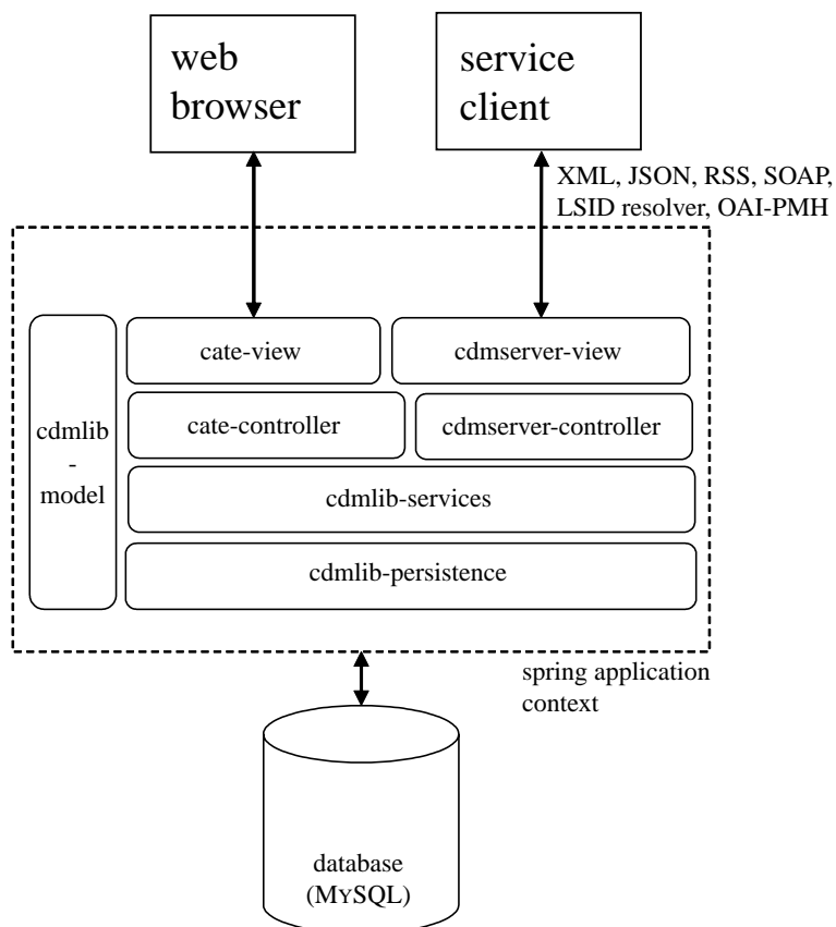
Figure 4. A high-level diagram summarizing the architecture of the CATE application. Each box represents a software component. CATE is built upon the EDIT CDM and Java Library; CDM objects are exchanged between layers of the application in response to a request from a client, such as a Web browser. The lowest layer, cdm lib-persistence, provides generic access to the database and the next layer, cdm lib-services, provides an application programming interface to the upper layers of the application. It is shared by both CATE and other software based upon the CDM. The CDM server exposes data as Web services (using the cdm server-controller and cdm server-view components); these allow other applications to access the data in the Web revision directly. In addition, CATE presents the data as a set of webpages, and provides the means for interacting with the data via a Web browser (using the cate -controller and cate -view components).
