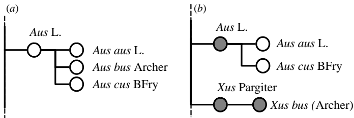
Figure 2. A specific example of a taxonomic change to a Web revision. (a) Sensu cate-aidae.org (2008): an imaginary revision of the family Aidae contains a genus Aus L. with three child taxa aus L., bus Archer and cus BFry. (b) Sensu Pargiter (2008) proposes that the existing classification be amended, specifically by creating a new genus Xus Pargiter, and by amending Aus L., transferring bus Archer into Xus . Circles represent taxon concepts, filled circles (in (b)) represent taxon concepts that are introduced or changed in Pargiter's proposal.
