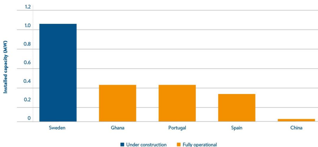
FIGURE 10: WAVE ENERGY INSTALLED CAPACITY IN OPERATION OR UNDER CONSTRUCTION
