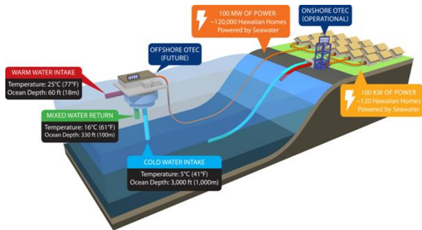
FIGURE 17: SCHEMATIC OF MAKAI OTEC PROJECT
