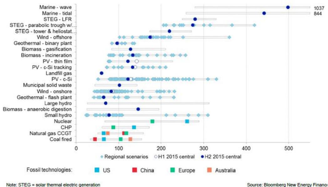
FIGURE 9: LEVELISED COST OF ELECTRICITY TECHNOLOGIES ($/MWH) FOR 2015
