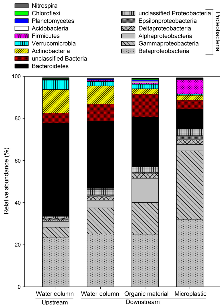
Fig. 4. Relative mean abundance of the 10 most abundant phyla based on 16S rRNA gene sequencing data for bacterial assemblages collected in 10 study streams. Proteobacteria is represented by relative abundance of classes.
