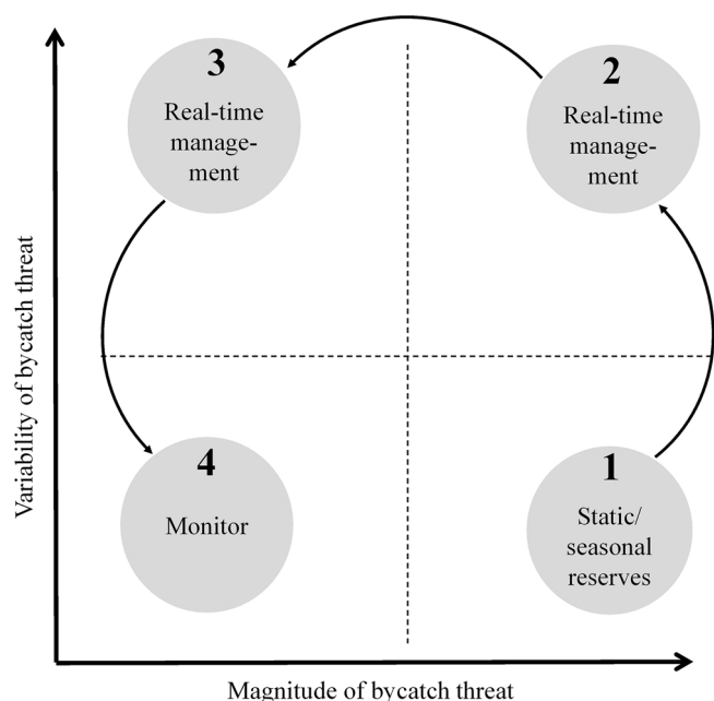
Fig. 5. Protection priority and possible management approaches for combinations of magnitude and variability of bycatch threat. For each month, pixels containing interactions are located on the plot using two values calculated across years of the time-series for a given species: magnitude of bycatch threat (the sum of threat across years) and variability of bycatch threat (the variance of threat across years). Priority 1 is highest, and 4 is lowest. Management implications for each priority category are relevant to portions of the year when pixels fall into that category. For example, pixels that move between top and second priority across months might be managed with seasonal no-take zones during months when they are top priority, and real-time management during the remainder of the year.
