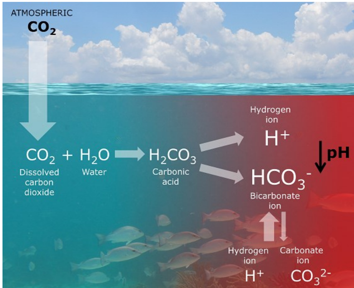
Fig. 1 Chemical reactions linked to \text{CO}_2 dissolution into the ocean. The different sizes of arrows in the bottom right corner indicate the shift of the chemical equilibrium as more \text{CO}_2 dissolves into seawater. Ultimately the process leads to an increase in \text{HCO}_3^- concentration at the expense of \text{CO}_3^{2-} concentration and a rise in \text{H}^+ concentration which causes a drop in pH (indicated by the red tint on the right side of the figure).
