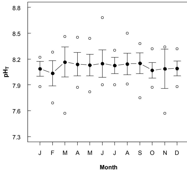
Fig. 4 Variation in pH T (pH on the total scale) in the Gullmar fjord (Sweden) based on monthly data between 1921 and 1987. Black dots represent average values (±SD); empty circles show maximum and minimum values. Modified from Dorey et al. (2013).
