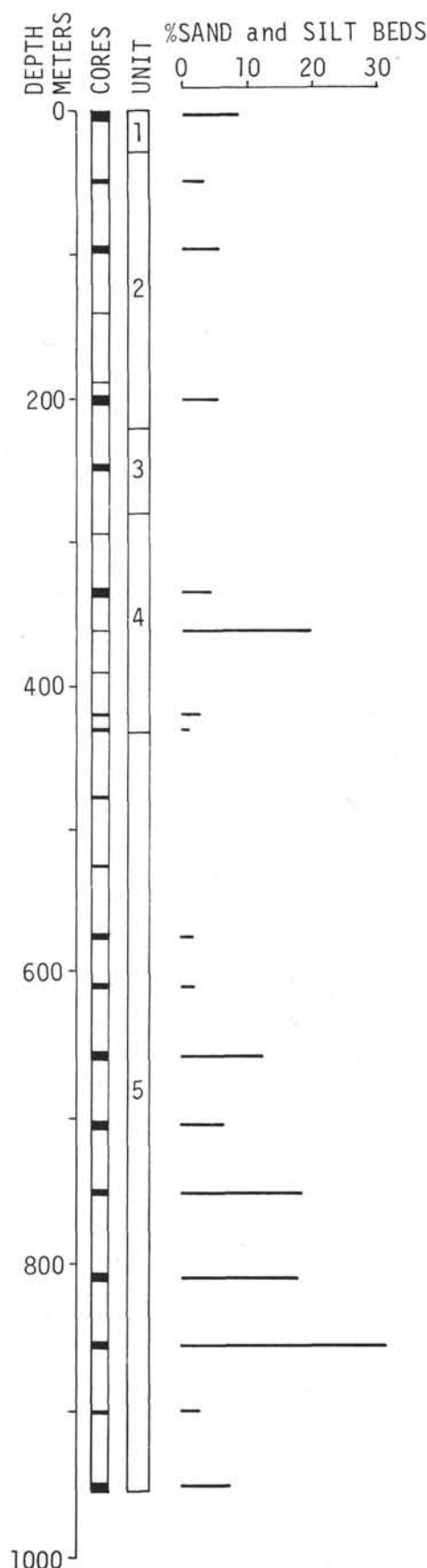
Figure 6. Distribution of sand and silt beds at Site 269.
