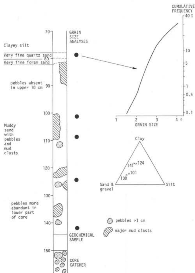
Figure 3. Sketch section of pebbly mud bed at base of 268-1-6, showing distribution of larger pebbles, and grain size analyses.
