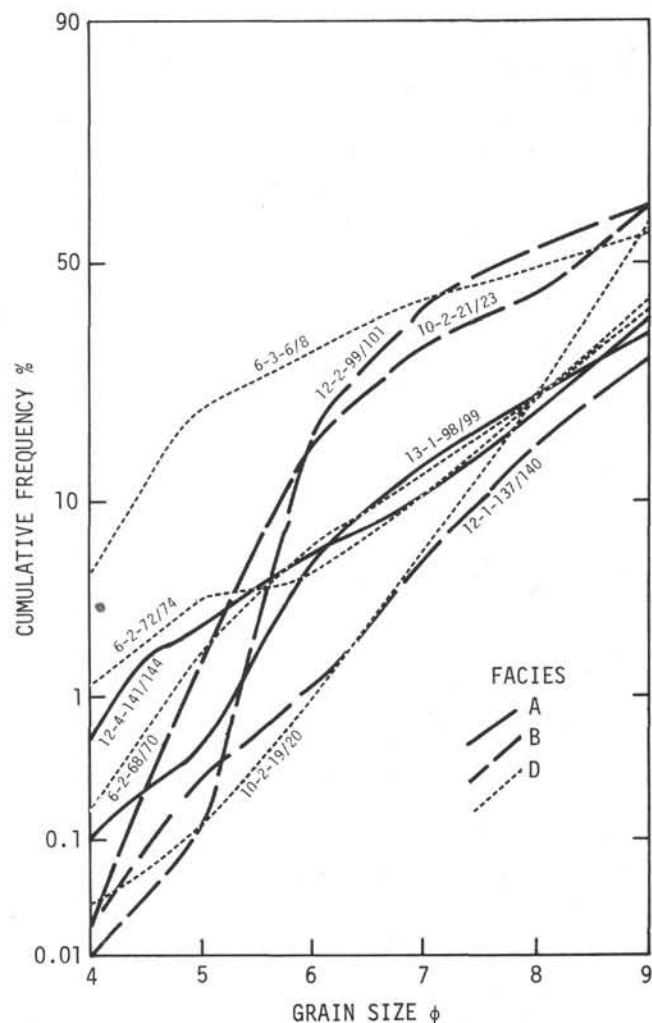
Figure 8. Grain size analyses of clay facies A, B, and D for the lower part of Hole 269A, determined by pipette analysis.
