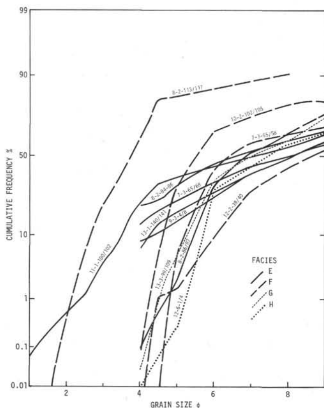
Figure 9. Grain size analyses of silts from the lower part of Hole 269A, determined by pipette analysis and sieving.
