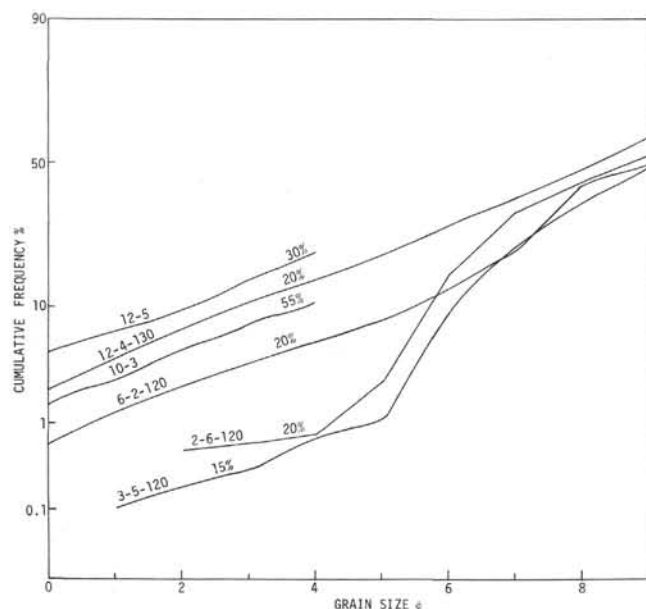
Figure 15. Grain size analyses of sediments in upper part of Site 274. Sediment mostly emplaced by ice rafting, but in part biogenic. Percentage of biogenic components (estimated from smear slides) is indicated.
