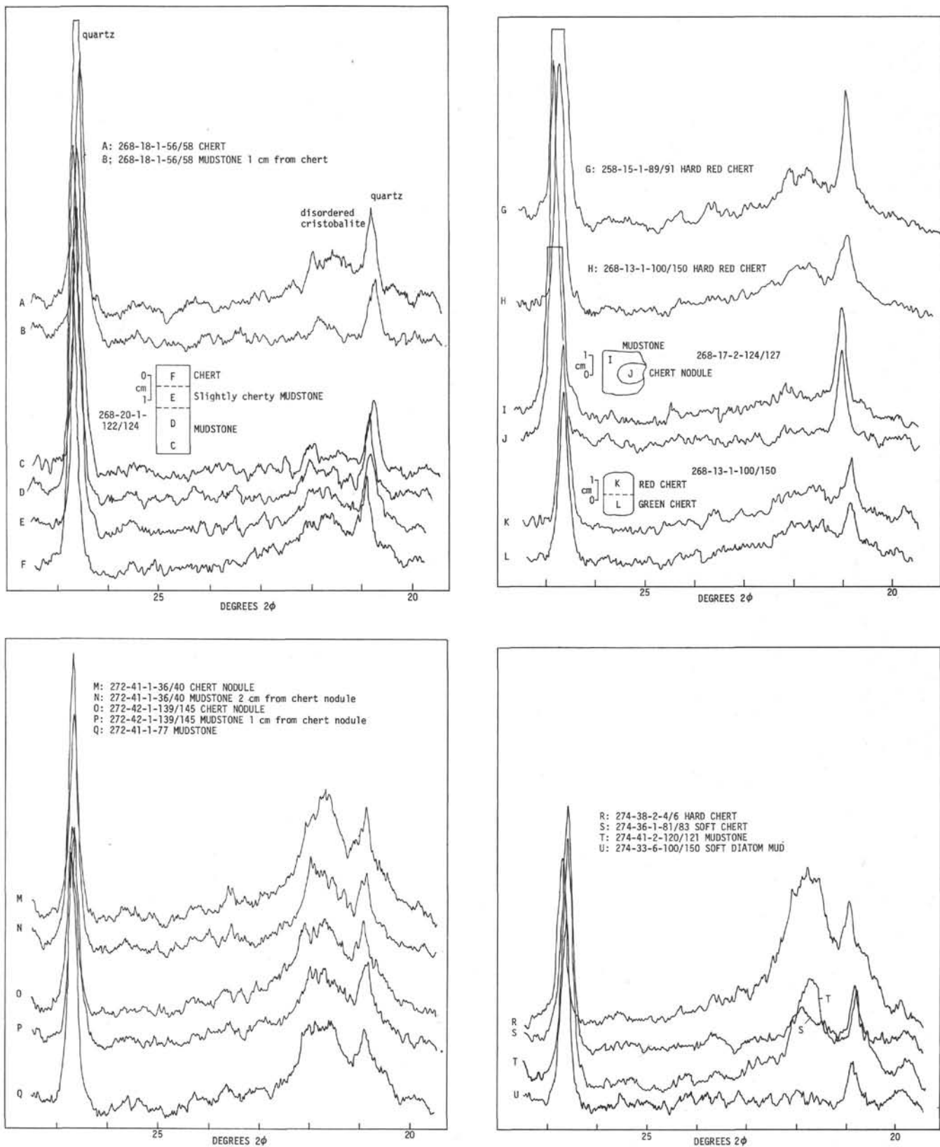
Figure 18. X-ray diffractograms of cherts and mudstones from Sites 268, 272, and 274, showing development of disordered cristobalite in different lithologies.
