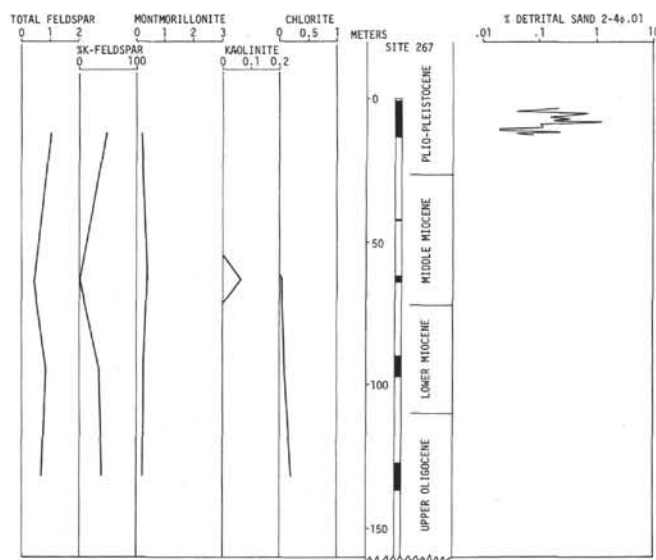
Figure 17. Variations in petrology with depth at Sites 267, 268, 269, and 274. Note that vertical scale is different for Site 269. The percent detrital sand (Table 4) is believed to represent ice-rafted sediment in most cases. Montmorillonite, kaolinite, and chlorite values from the less than 2 M X-ray diffraction data of Zemmels (Chapter 00), normalized to mica = 1.0. Total feldspar, and percentage of feldspar that is K feldspar, based on bulk X-ray diffraction analysis by Zemmels, normalized to quartz = 1.0. Percent cristobalite based on bulk X-ray diffraction data. Note that adjacent data points have been joined purely to facilitate reading of the graph. No geologic predictions are intended. Presence of chert based on visual core description. Presence of volcanic glass (generally in trace amounts) based on smear slide identifications. Note the probability of operator variance in the recognition of volcanic glass.
