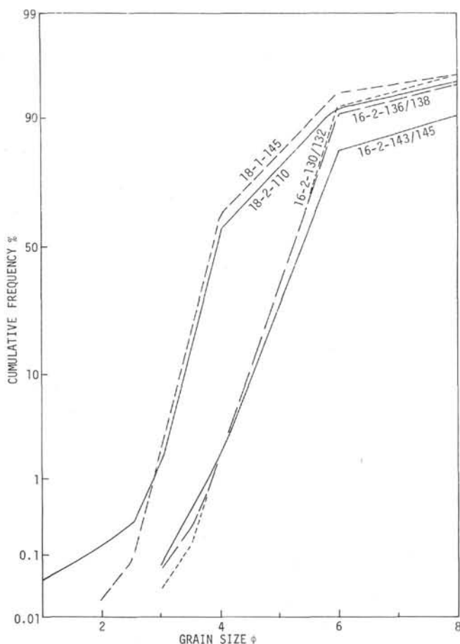
Figure 14. Grain size analyses of turbidite silt beds from Site 274. (a) Near base, and from upper part of 2.7-meter thick sand bed in Core 18 (base at 274-18-2, 120). Compare with Table 3. (b) Samples from middle and lower part of a 40-cm-thick silt bed, grading up into 50 cm alternating silt and clay (base at 274-16-2, 146).
