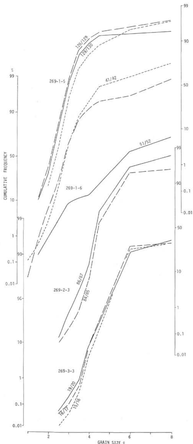
Figure 7. Grain size analyses of turbidite sand and silt beds from upper part of Site 269, determined by pipette analysis and sieving.
