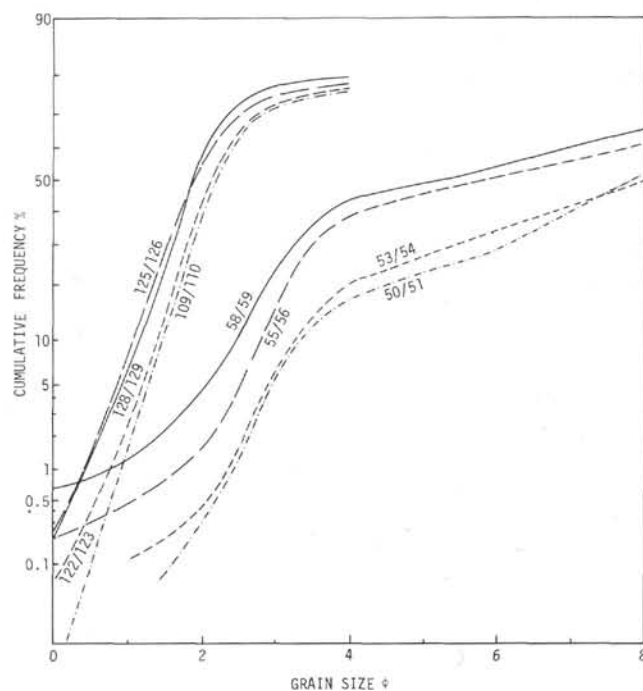
Figure 2. Grain size analyses of two turbidite sand beds from upper part of Site 268. (a) bed with base at 268-2-2, 130 cm. (b) bed with base at 268-5-2, 59 cm.
