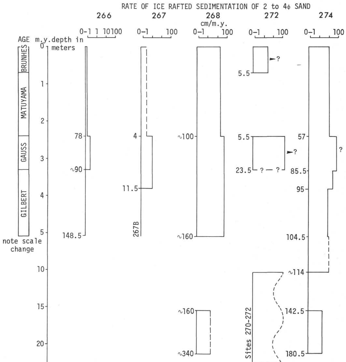
Figure 16. Rates of accumulation of ice rafted 2 to 40 sand, in cm/m.y. Based on core thicknesses, abundance of sand (Table 4), and available biostratigraphic data. The biostratigraphic summary shown in Figure 3 of Chapter 1 (Introduction) has been used, with the following exceptions: Site 266: the assignment of the base of the Gauss is speculative. Site 267: dating of Core 1A (4-13 m) as Gauss disconformable on upper Gilbert is speculative, partly based on Radiolaria, and silicoflagellates (Ciesielski, personal communication). Hole 272: recognition of Brunhes part of sequence based on lithologic correlation with the cores of Fillon (1972) (see Barrett, Chapter 22). Note the Brunhes thickness is very uncertain. Hole 274: Position of top of Gauss uncertain; it may be lower than shown, in which case the Gauss might not be represented by recovered core. Detailed dating of Gilbert based mainly on silicoflagellates (Ciesielski, personal communication). Base of the upper Miocene may have been picked too low, so that the higher upper Miocene sedimentation rate may also apply to the topmost middle Miocene.
