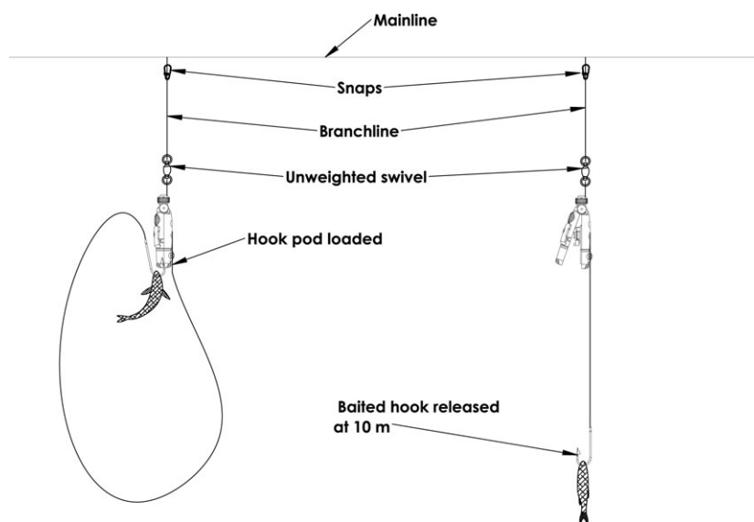
Figure 2 The Hookpod in situ prior to and after the pressure release mechanism opens the pod.
