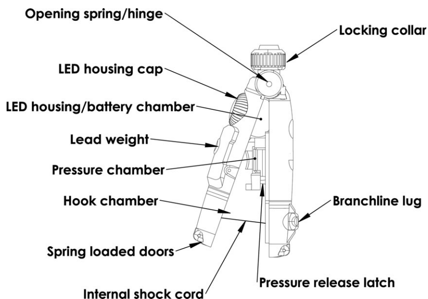
Figure 1 Components of the Hookpod.
