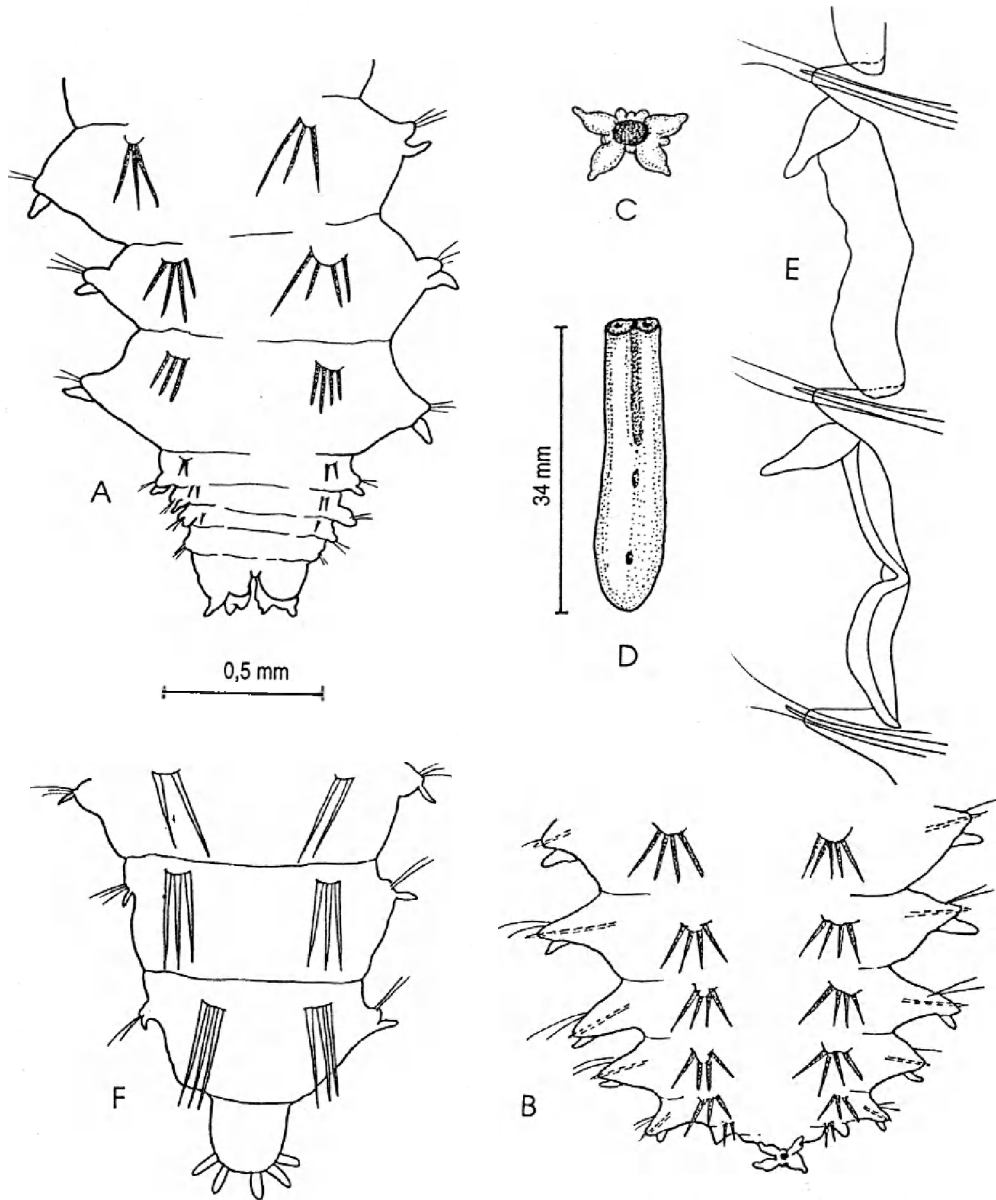
Fig. 3. Trochochaeta carica (BIRULA). A, B. Posterior ends of different specimens, dorsal view. C. Anus encircled by lobes. D. Fragment of tube, lower part. E. Abdominal neuropodia. (A-D, specimens from the Gulf of Ob; E, from the Chaun Bay). Trochochaeta sp. F. Posterior end, dorsal view. (Specimen from the Saint John River Estuary).
