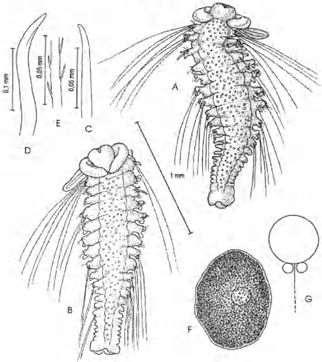
Fig. 4. Trochochaeta carica (BIRULA). A. Larva, dorsal view. B. The same, ventral view. C. Seta from segment 2. D. Seta from segment 3. E. Detail of provisional swimming seta. F. Egg. G. Sperm. (Specimens from the Gulf of Ob).
