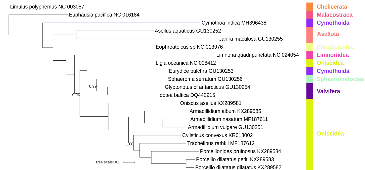
Fig 2. Mitochondrial phylogenomics of Isopoda: Bayesian inference analysis. The analysis was conducted using nucleotide sequences of all genes. Limulus polyphemus (branch cropped) and Euphausia pacifica are outgroups. Scale bar corresponds to the estimated number of substitutions per site. Bayesian posterior probability values (lower than 1.0) are shown next to corresponding nodes. GenBank accession numbers are shown next to species names. Taxonomic rank (suborder/superfamily) is shown to the right. Coloured branches highlight paraphyly.
