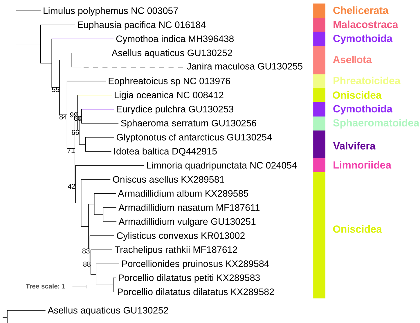
Fig 3. Mitochondrial phylogenomics of Isopoda: Maximum likelihood analysis. The analysis was conducted using nucleotide sequences of all genes. Limulus polyphemus and Euphausia pacifica are outgroups. Scale bar corresponds to the estimated number of substitutions per site. Bootstrap support values (lower than 100) are shown next to corresponding nodes. GenBank accession numbers are shown next to species names. Taxonomic rank (suborder/superfamily) is shown to the right. Coloured branches highlight paraphyly. Janira maculosa branch (dashed line) is shortened, with its original size shown below the phylogram.
