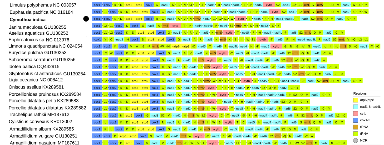
Fig 1. Gene order in isopod mitogenomes. The newly sequenced species, Cymothoa indica , is bolded and marked with a black dot. GenBank accession numbers are shown next to the species names, and gene legend is incorporated in the figure. Two outgroups, Limulus polyphemus and Euphausia pacifica , are also shown.
