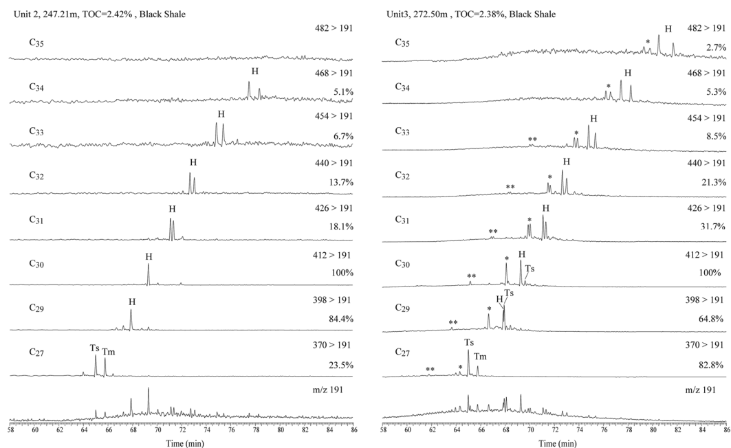
Figure 4. Partial m/z 191 mass chromatograms (bottom) and MRM data showing the C_{27} to C_{35} hopane and diahopane series in Unit 3 (272.5 m) and the overlying Unit 2 (247.21 m) (H: C_{30}17\alpha(H) -hopane; *17\alpha(H) -diahopanes ( C_{27} and C_{29} - C_{35} ); **C_{30} early-eluting rearranged hopanes).
