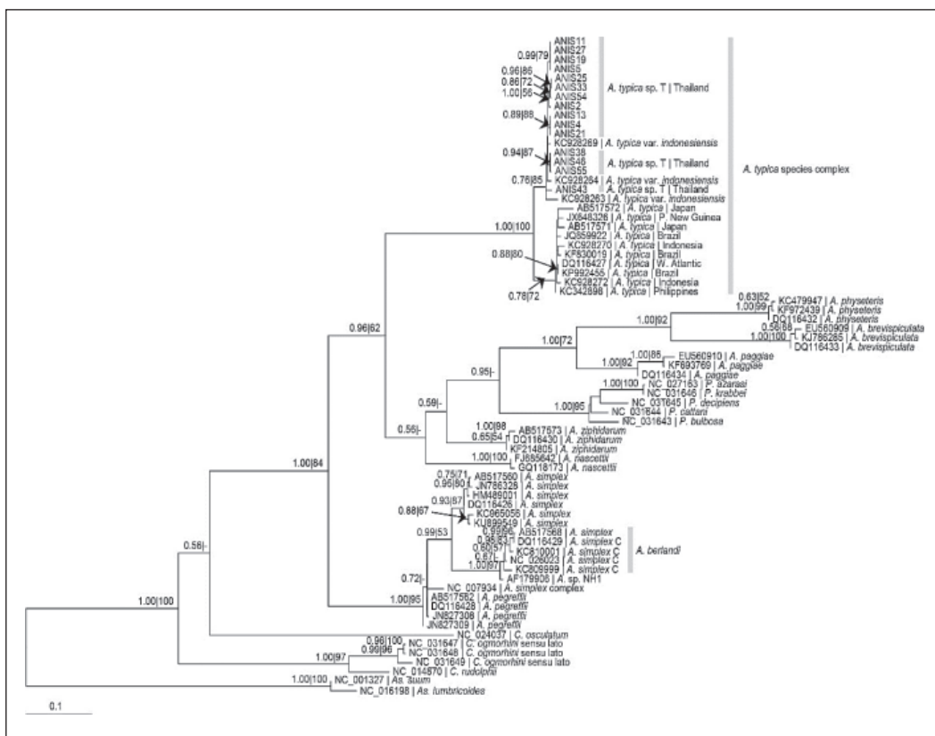
Figure 1. Bayesian inference (BI) and maximum likelihood (ML) phylogenetic tree of Anisakis taxa and related anisakid genera based on mitochondrial cytochrome c oxidase subunit II nucleotide sequences. Anisakis typica sp. T from Thailand and A. typica var. indonesiensis from Indonesia formed a lineage distinct from A. typica sensu stricto. A., Anisakis ; As., Ascaris ; C., Contracaecum ; P., Pseudoterranova .
