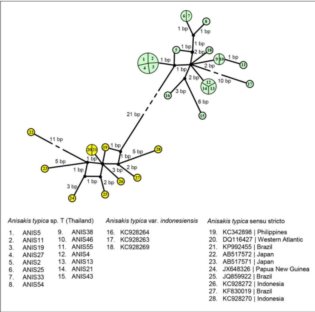
Figure 2. Haplotype networks of Anisakis typica sp. T, A. typica var. indonesiensis and A. typica sensu stricto based on mitochondrial cytochrome c oxidase subunit II nucleotide sequences generated by NETWORK software. MtDNA cox2 haplotypes of A. typica complex comprising A. typica sp. T and A. typica var. indonesiensis were distinctly separated from those of A. typica sensu stricto. Circle represents haplotype and sizes are relative to the number of individuals sharing the specific haplotype.
